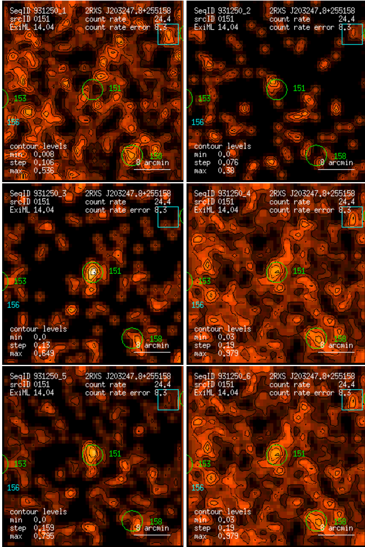
Figure 151: RASS 931250: detection 0151: band rate images, Gaussian filter: (1) PSPPC channels 11 – 41, (2) 52 – 90, (3) 91 – 201, (4) 11 – 235, (5) 52 – 201, (6) 11 – 201. Broad band rates in counts/ks. Band rate contour levels in counts/ks/arcmin 2 .
