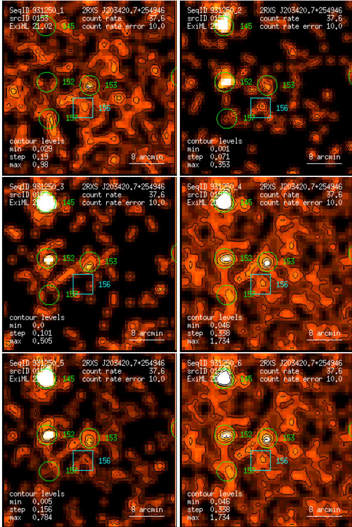
Figure 153: RASS 931250: detection 0153: band rate images, Gaussian filter: (1) PSPC channels 11 – 41, (2) 52 – 90, (3) 91 – 201, (4) 11 – 235, (5) 52 – 201, (6) 11 – 201. Broad band rates in counts/ks. Band rate contour levels in counts/ks/arcmin 2 .
