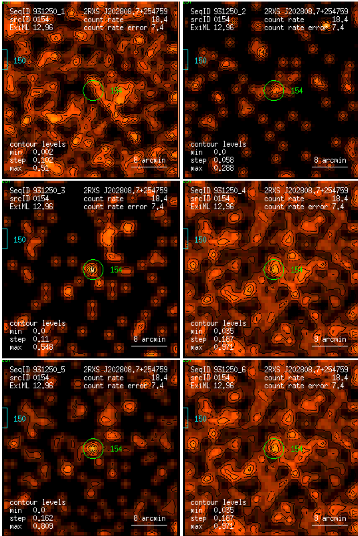
Figure 154: RASS 931250: detection 0154: band rate images, Gaussian filter: (1) PSPC channels 11 – 41, (2) 52 – 90, (3) 91 – 201, (4) 11 – 235, (5) 52 – 201, (6) 11 – 201. Broad band rates in counts/ks. Band rate contour levels in counts/ks/arcmin 2 .
