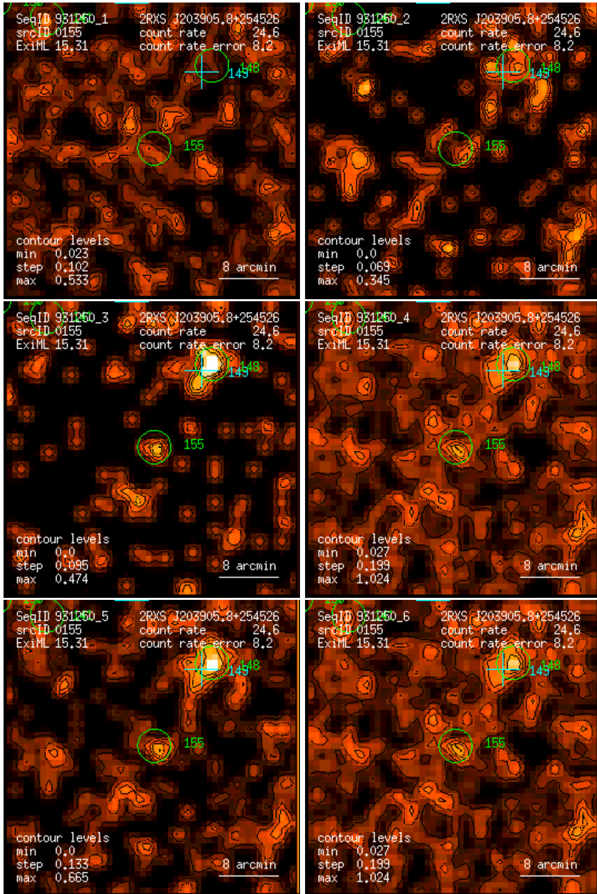
Figure 155: RASS 931250: detection 0155: band rate images, Gaussian filter: (1) PSPC channels 11 – 41, (2) 52 – 90, (3) 91 – 201, (4) 11 – 235, (5) 52 – 201, (6) 11 – 201. Broad band rates in counts/ks. Band rate contour levels in counts/ks/arcmin 2 .
