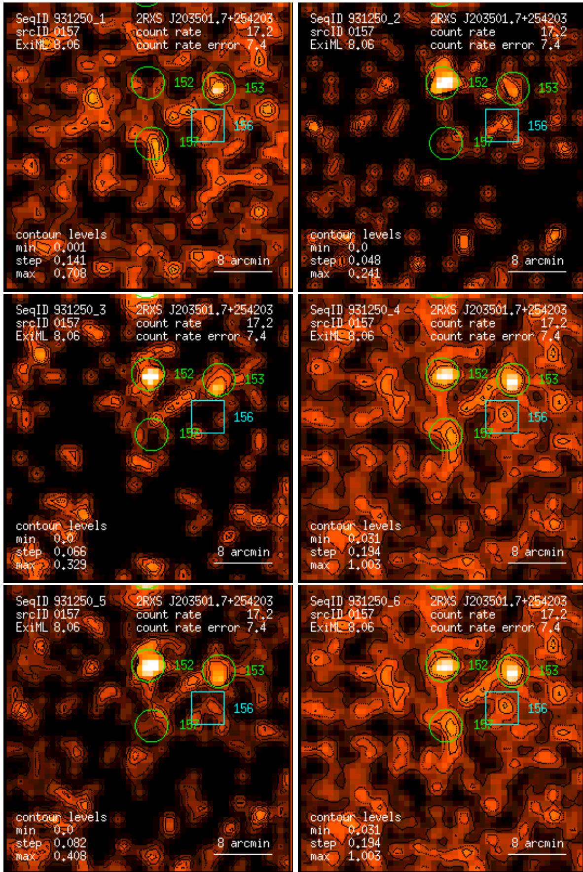
Figure 157: RASS 931250: detection 0157: band rate images, Gaussian filter: (1) PSPC channels 11 – 41, (2) 52 – 90, (3) 91 – 201, (4) 11 – 235, (5) 52 – 201, (6) 11 – 201. Broad band rates in counts/ks. Band rate contour levels in counts/ks/arcmin 2 .
