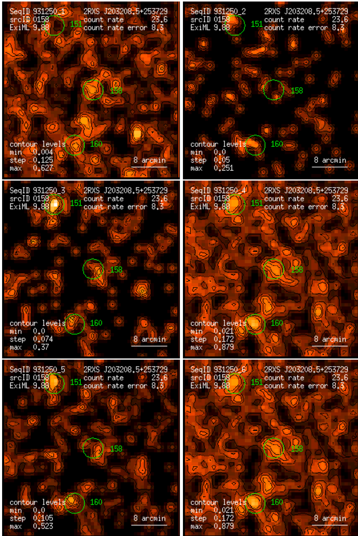
Figure 158: RASS 931250: detection 0158: band rate images, Gaussian filter: (1) PSPC channels 11 – 41, (2) 52 – 90, (3) 91 – 201, (4) 11 – 235, (5) 52 – 201, (6) 11 – 201. Broad band rates in counts/ks. Band rate contour levels in counts/ks/arcmin 2 .
