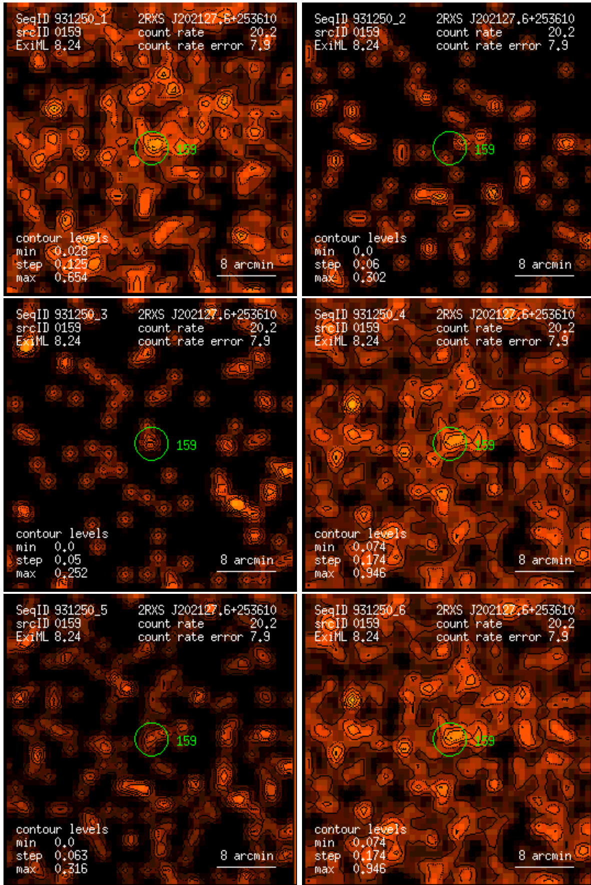
Figure 159: RASS 931250: detection 0159: band rate images, Gaussian filter: (1) PSPC channels 11 – 41, (2) 52 – 90, (3) 91 – 201, (4) 11 – 235, (5) 52 – 201, (6) 11 – 201. Broad band rates in counts/ks. Band rate contour levels in counts/ks/arcmin 2 .
