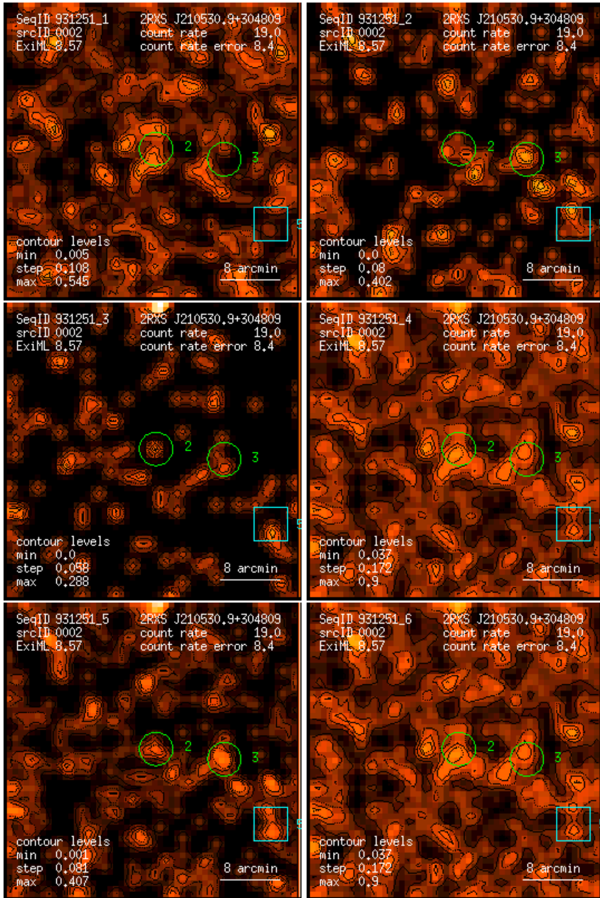
Figure 2: RASS 931251: detection 0002: band rate images, Gaussian filter: (1) PSPC channels 11 – 41, (2) 52 – 90, (3) 91 – 201, (4) 11 – 235, (5) 52 – 201, (6) 11 – 201. Broad band rates in counts/ks. Band rate contour levels in counts/ks/arcmin 2 .
