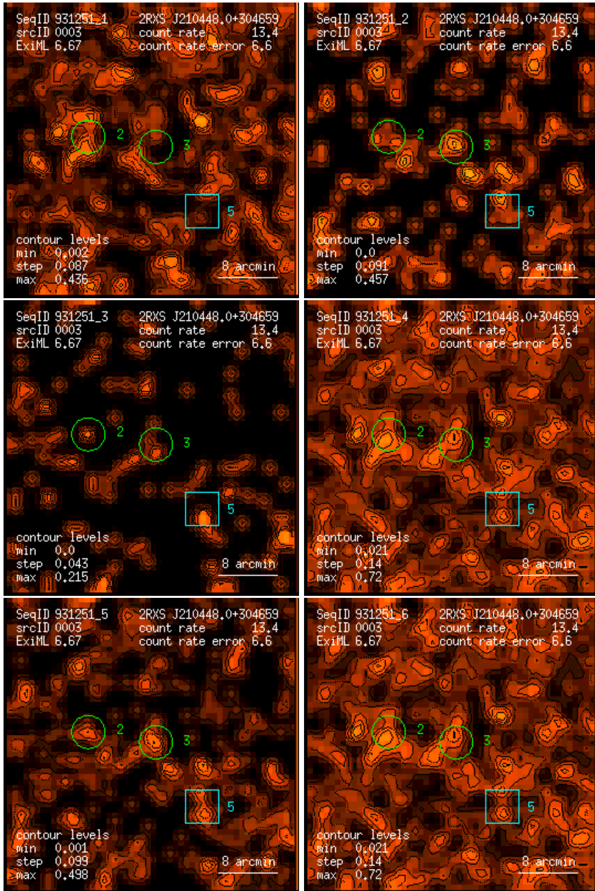
Figure 3: RASS 931251: detection 0003: band rate images, Gaussian filter: (1) PSPC channels 11 – 41, (2) 52 – 90, (3) 91 – 201, (4) 11 – 235, (5) 52 – 201, (6) 11 – 201. Broad band rates in counts/ks. Band rate contour levels in counts/ks/arcmin 2 .
