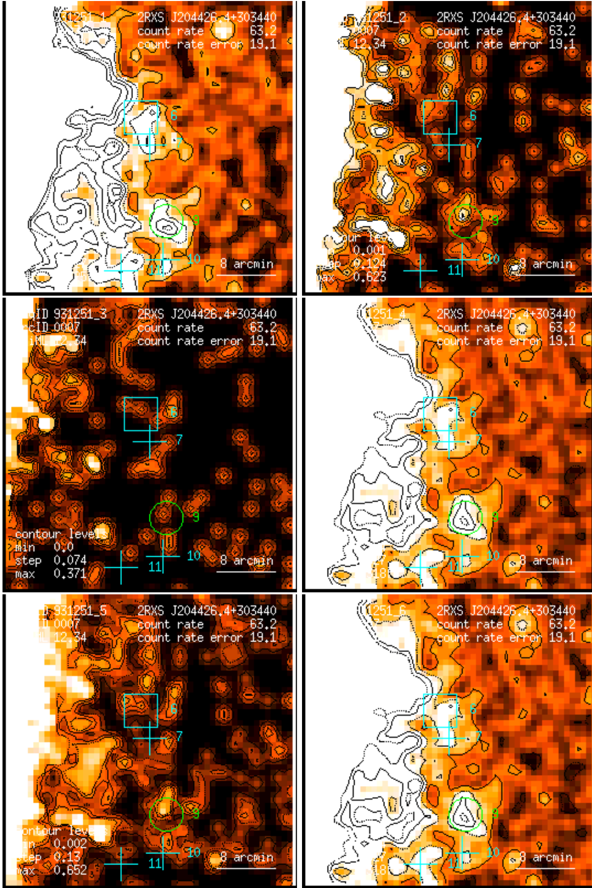
Figure 7: RASS 931251: detection 0007: band rate images, Gaussian filter: (1) PSPC channels 11 – 41, (2) 52 – 90, (3) 91 – 201, (4) 11 – 235, (5) 52 – 201, (6) 11 – 201. Broad band rates in counts/ks. Band rate contour levels in counts/ks/arcmin 2 .
