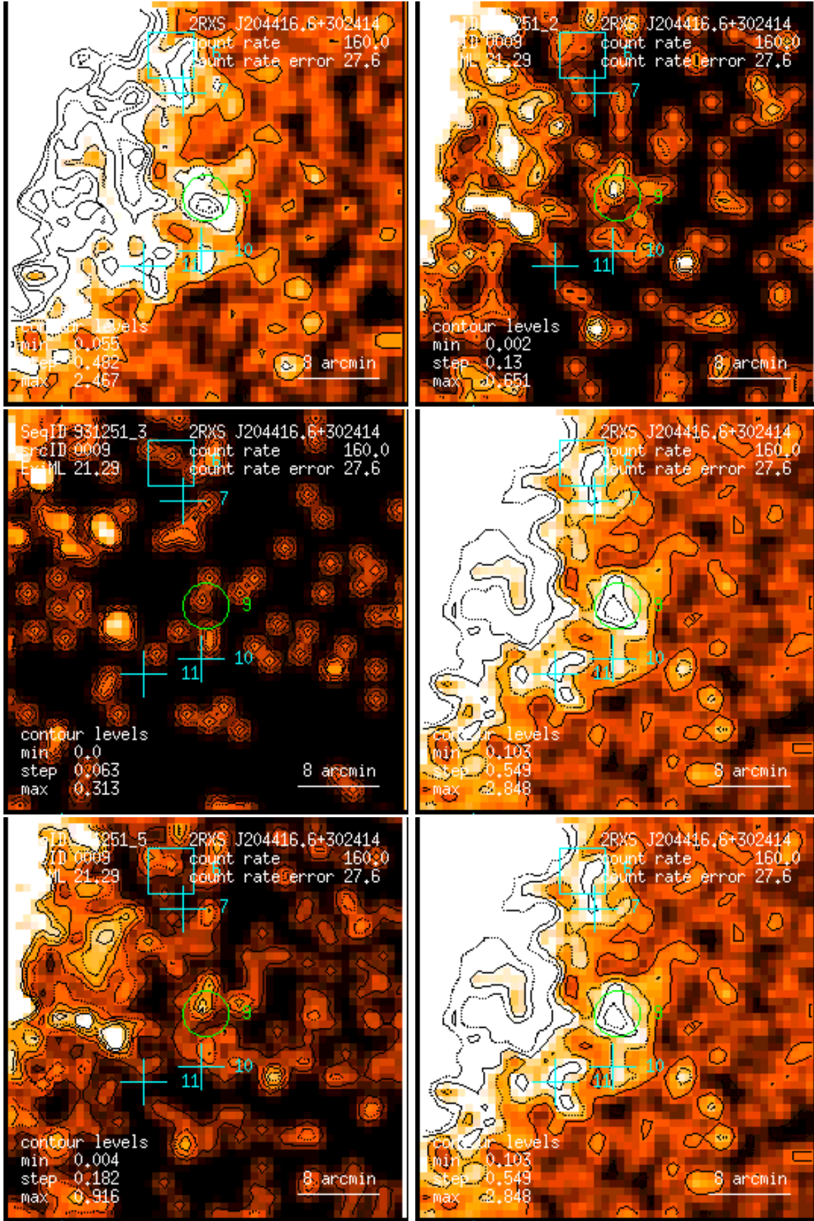
Figure 9: RASS 931251: detection 0009: band rate images, Gaussian filter: (1) PSPC channels 11 – 41, (2) 52 – 90, (3) 91 – 201, (4) 11 – 235, (5) 52 – 201, (6) 11 – 201. Broad band rates in counts/ks. Band rate contour levels in counts/ks/arcmin 2 .
