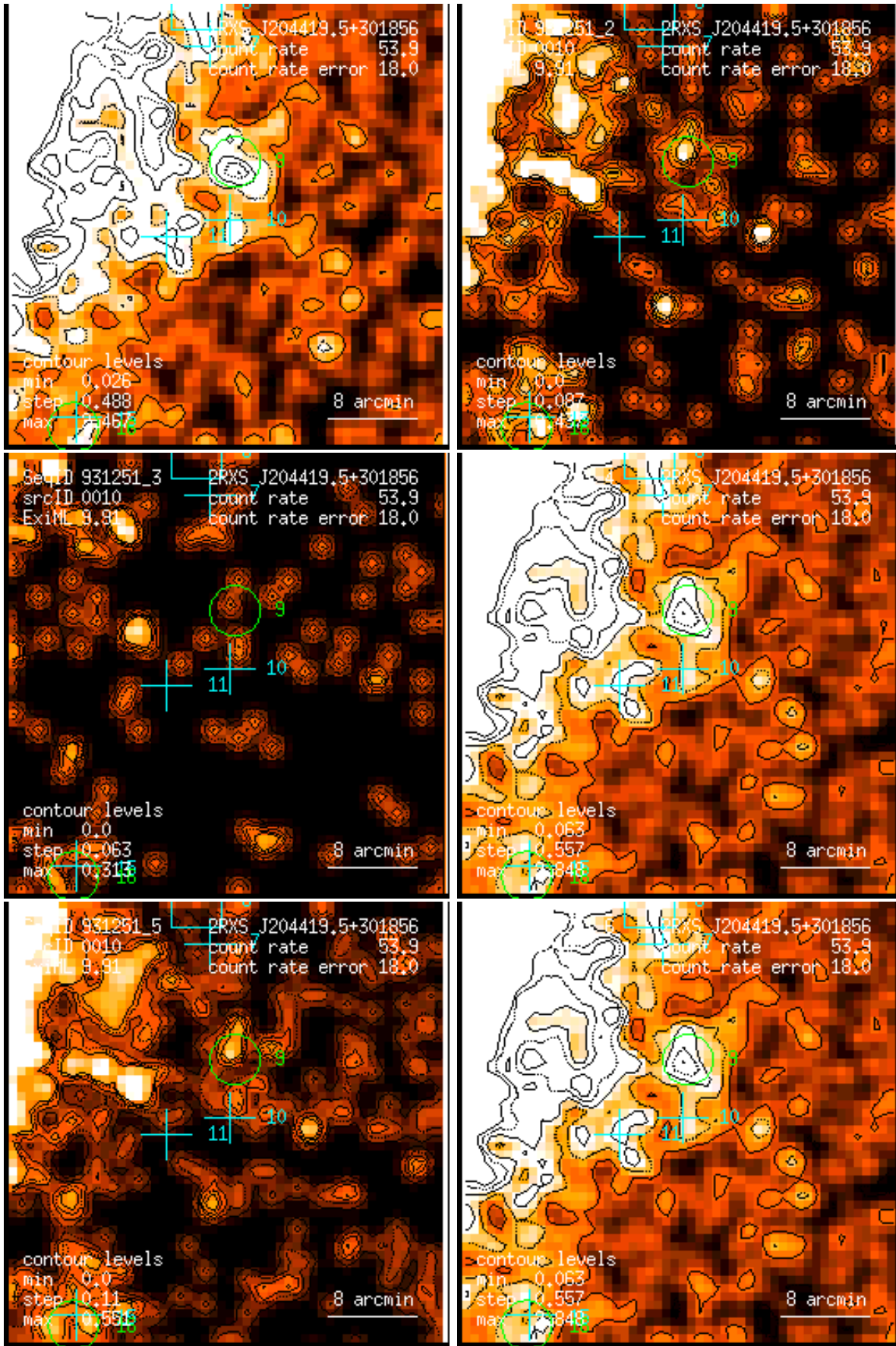
Figure 10: RASS 931251: detection 0010: band rate images, Gaussian filter: (1) PSPC channels 11 – 41, (2) 52 – 90, (3) 91 – 201, (4) 11 – 235, (5) 52 – 201, (6) 11 – 201. Broad band rates in counts/ks. Band rate contour levels in counts/ks/arcmin 2 .
