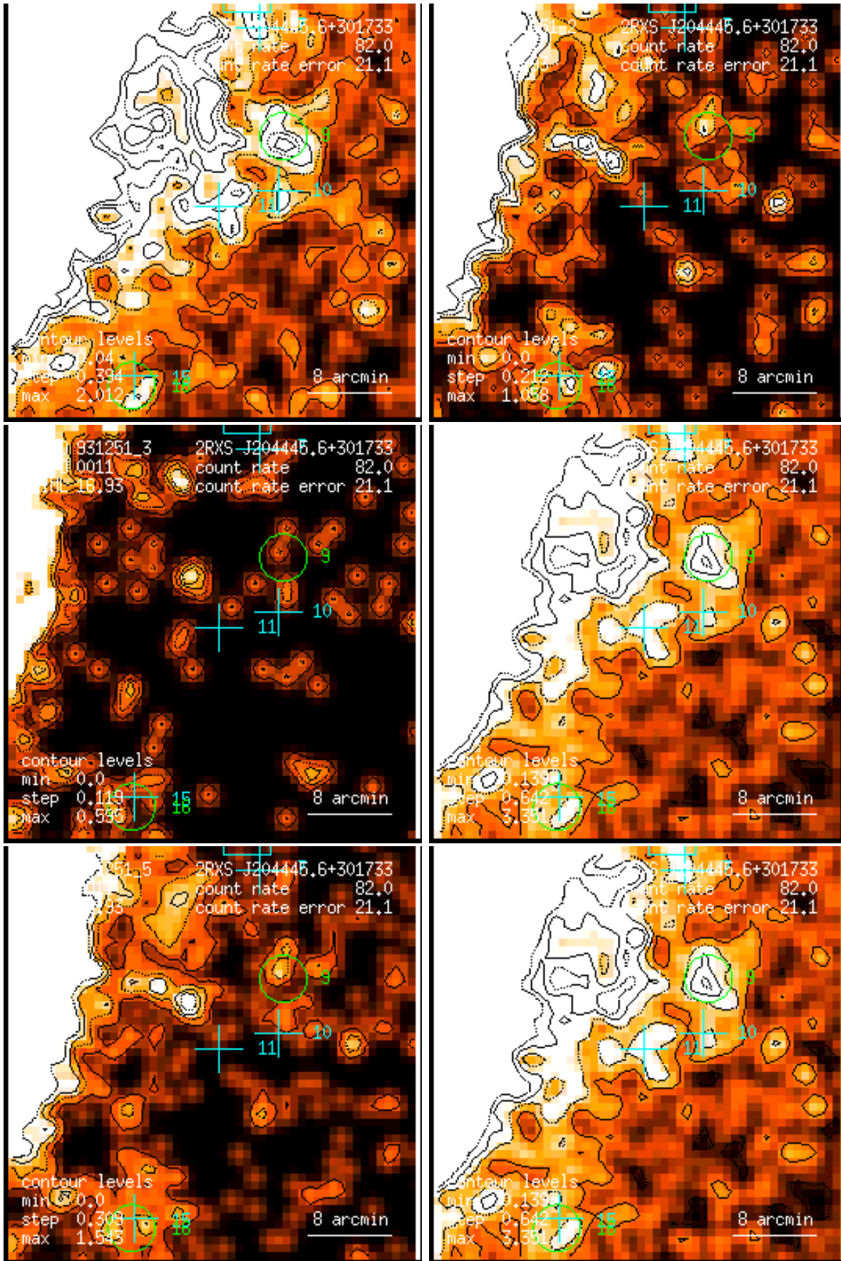
Figure 11: RASS 931251: detection 0011: band rate images, Gaussian filter: (1) PSPC channels 11 – 41, (2) 52 – 90, (3) 91 – 201, (4) 11 – 235, (5) 52 – 201, (6) 11 – 201. Broad band rates in counts/ks. Band rate contour levels in counts/ks/arcmin 2 .
