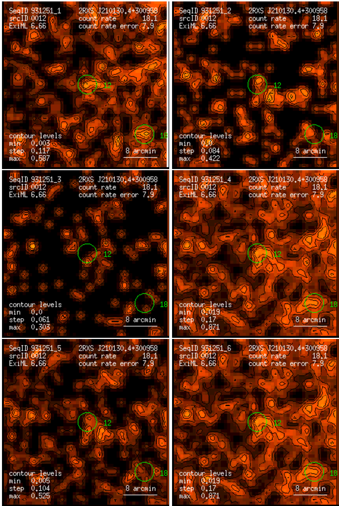
Figure 12: RASS 931251: detection 0012: band rate images, Gaussian filter: (1) PSPC channels 11 – 41, (2) 52 – 90, (3) 91 – 201, (4) 11 – 235, (5) 52 – 201, (6) 11 – 201. Broad band rates in counts/ks. Band rate contour levels in counts/ks/arcmin 2 .
