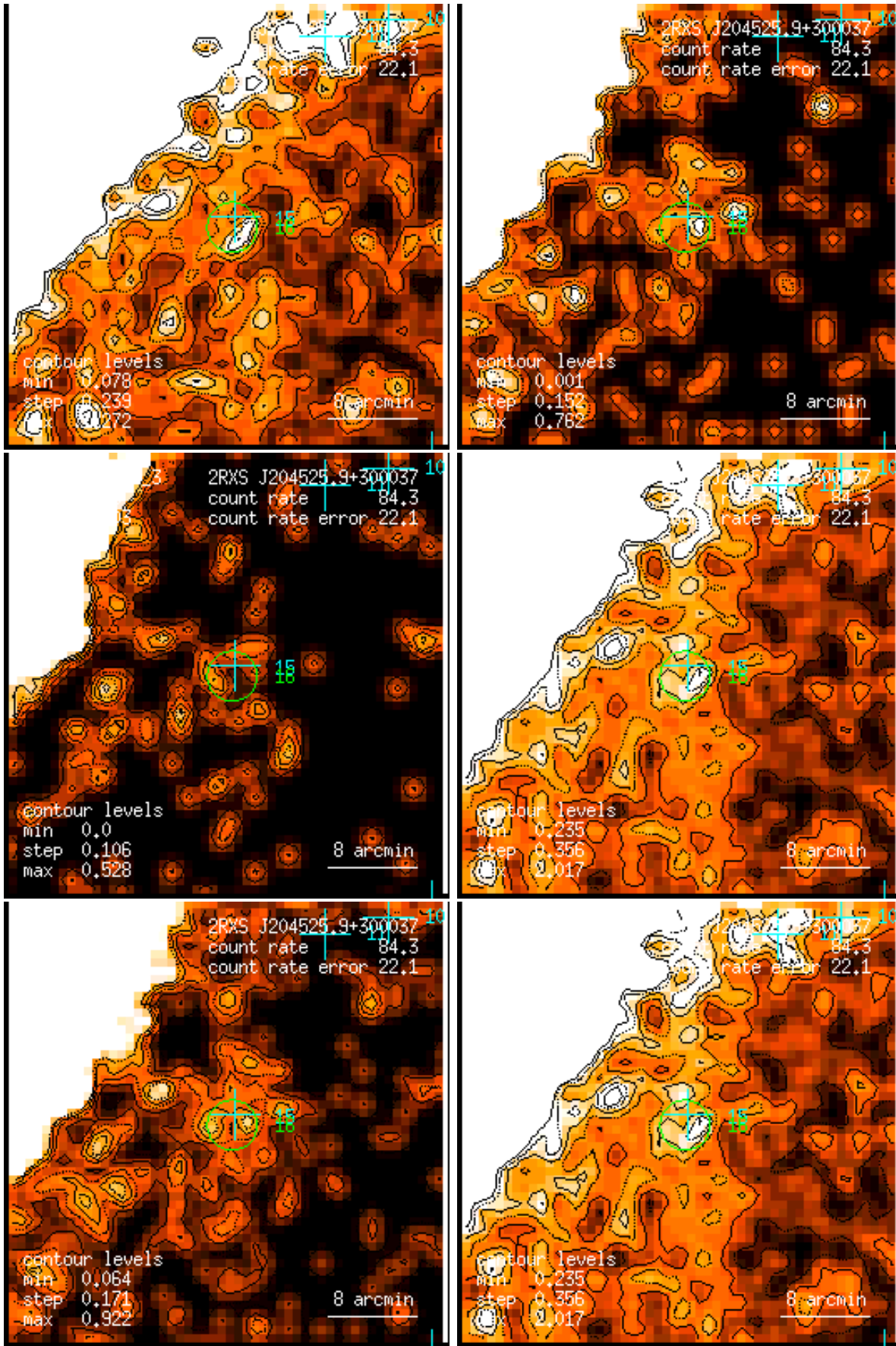
Figure 16: RASS 931251: detection 0016: band rate images, Gaussian filter: (1) PSPC channels 11 – 41, (2) 52 – 90, (3) 91 – 201, (4) 11 – 235, (5) 52 – 201, (6) 11 – 201. Broad band rates in counts/ks. Band rate contour levels in counts/ks/arcmin 2 .
