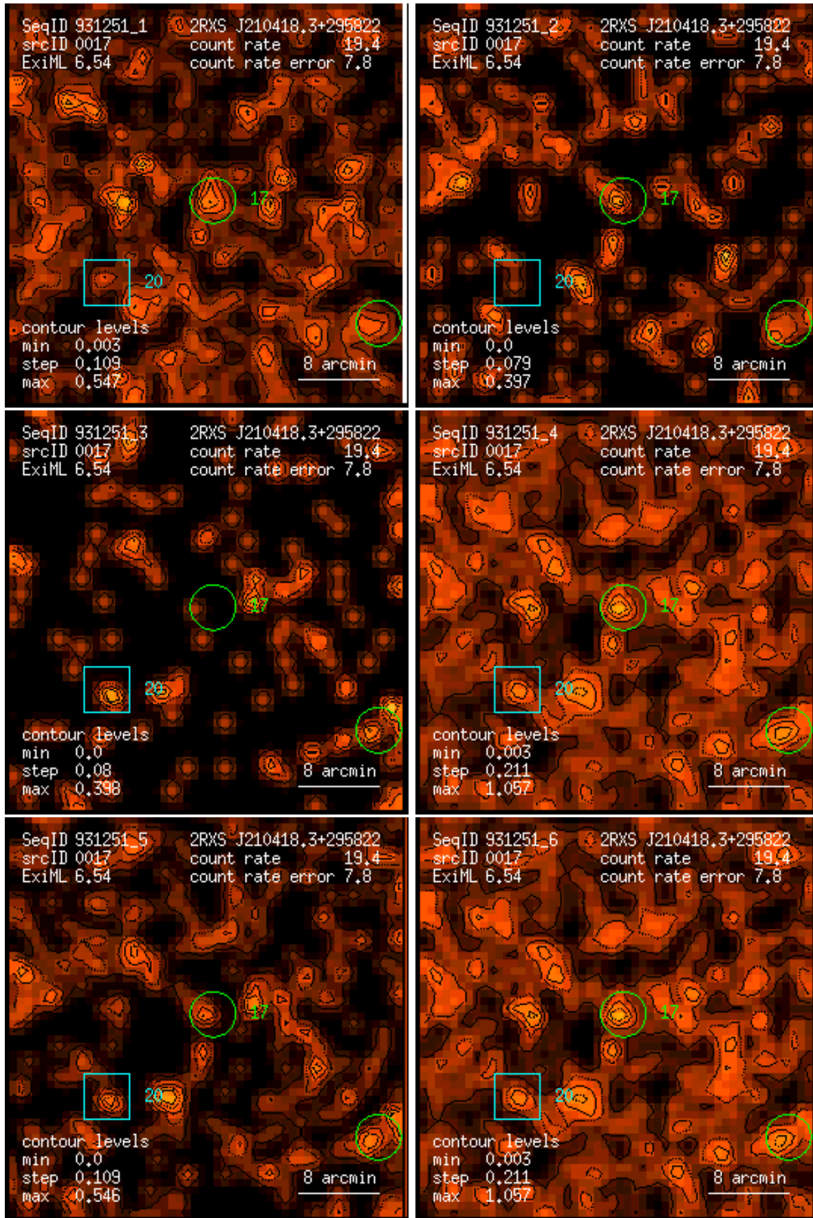
Figure 17: RASS 931251: detection 0017: band rate images, Gaussian filter: (1) PSPC channels 11 – 41, (2) 52 – 90, (3) 91 – 201, (4) 11 – 235, (5) 52 – 201, (6) 11 – 201. Broad band rates in counts/ks. Band rate contour levels in counts/ks/arcmin 2 .
