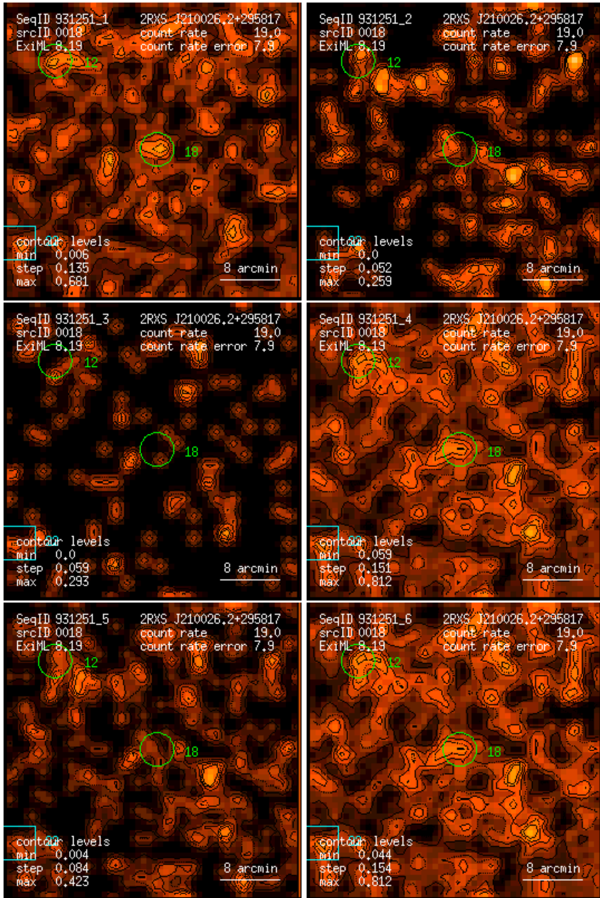
Figure 18: RASS 931251: detection 0018: band rate images, Gaussian filter: (1) PSPC channels 11 – 41, (2) 52 – 90, (3) 91 – 201, (4) 11 – 235, (5) 52 – 201, (6) 11 – 201. Broad band rates in counts/ks. Band rate contour levels in counts/ks/arcmin 2 .
