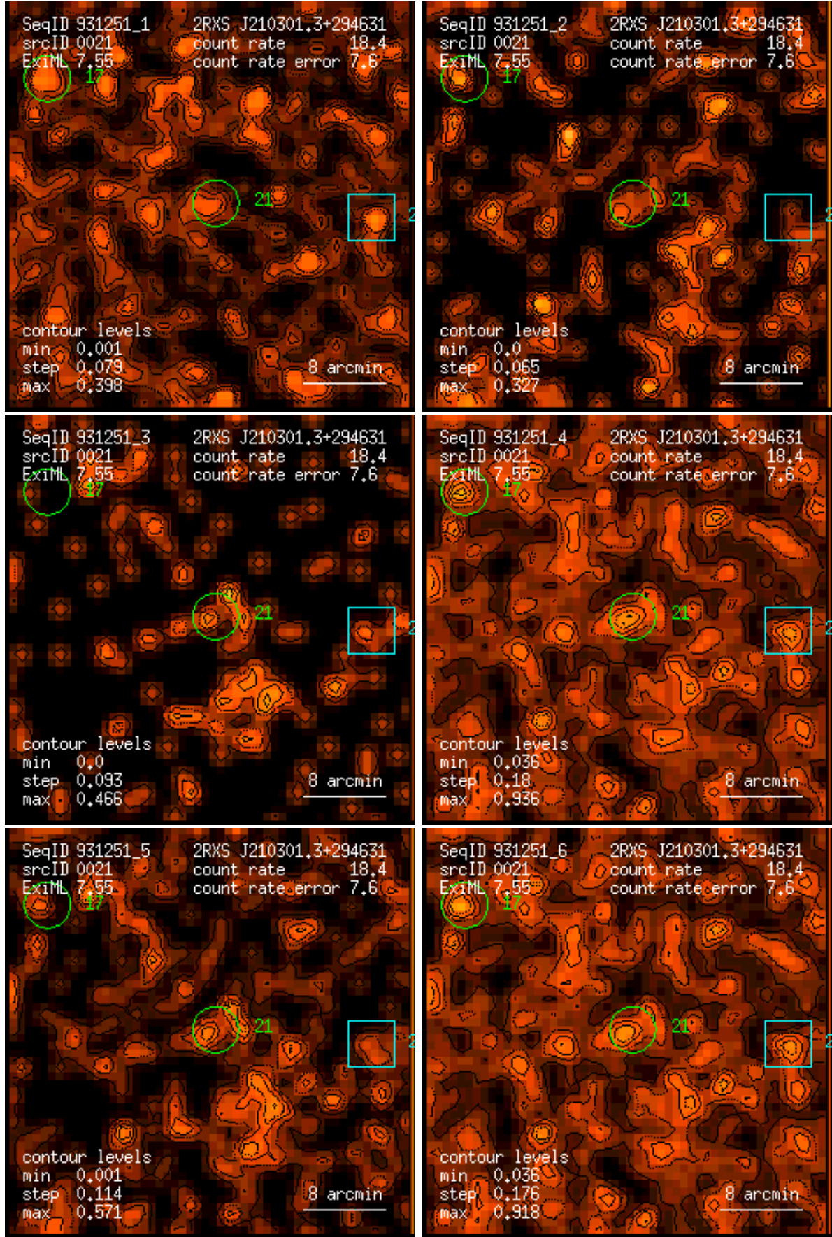
Figure 21: RASS 931251: detection 0021: band rate images, Gaussian filter: (1) PSPC channels 11 – 41, (2) 52 – 90, (3) 91 – 201, (4) 11 – 235, (5) 52 – 201, (6) 11 – 201. Broad band rates in counts/ks. Band rate contour levels in counts/ks/arcmin 2 .
