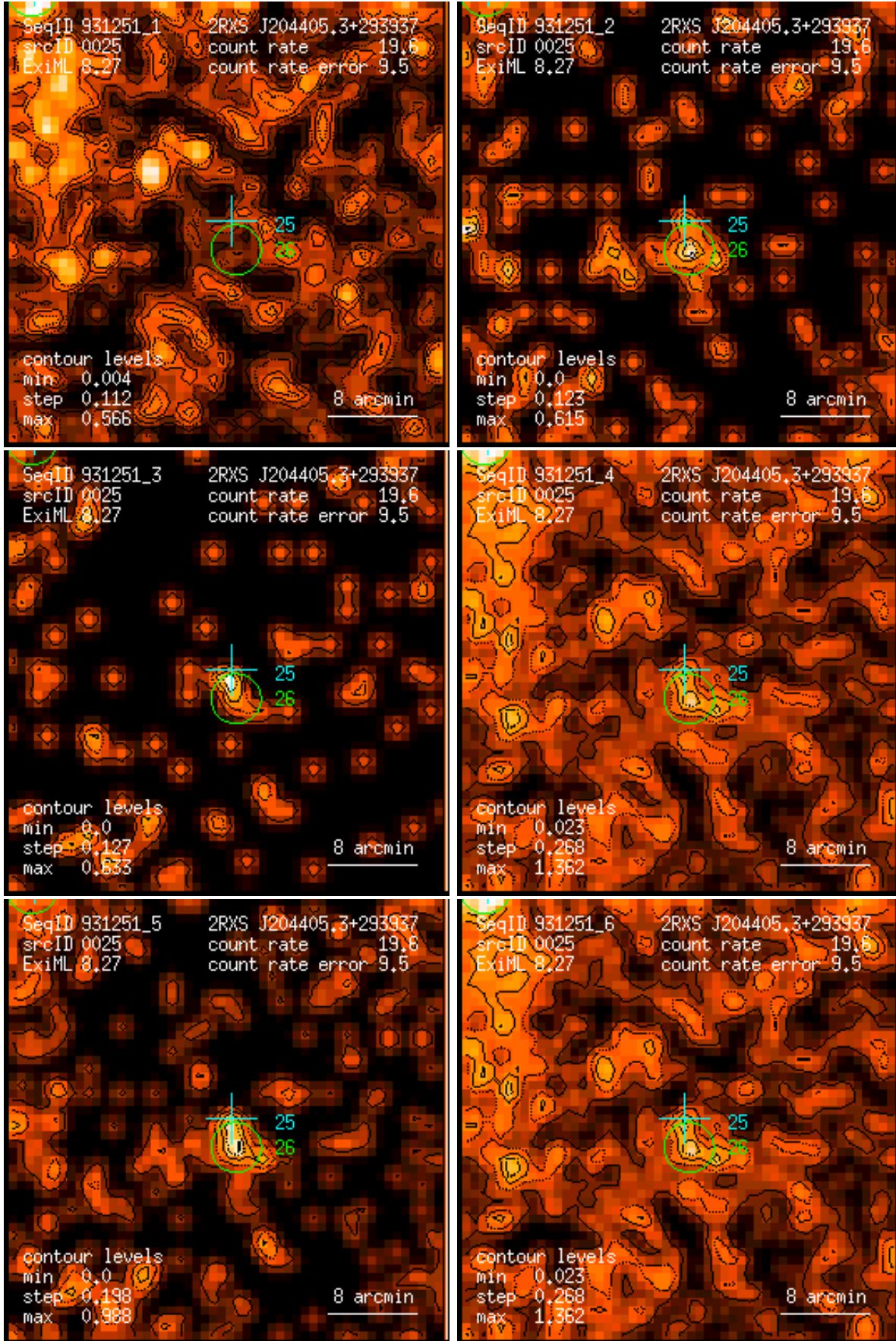
Figure 25: RASS 931251: detection 0025: band rate images, Gaussian filter: (1) PSPC channels 11 – 41, (2) 52 – 90, (3) 91 – 201, (4) 11 – 235, (5) 52 – 201, (6) 11 – 201. Broad band rates in counts/ks. Band rate contour levels in counts/ks/arcmin 2 .
