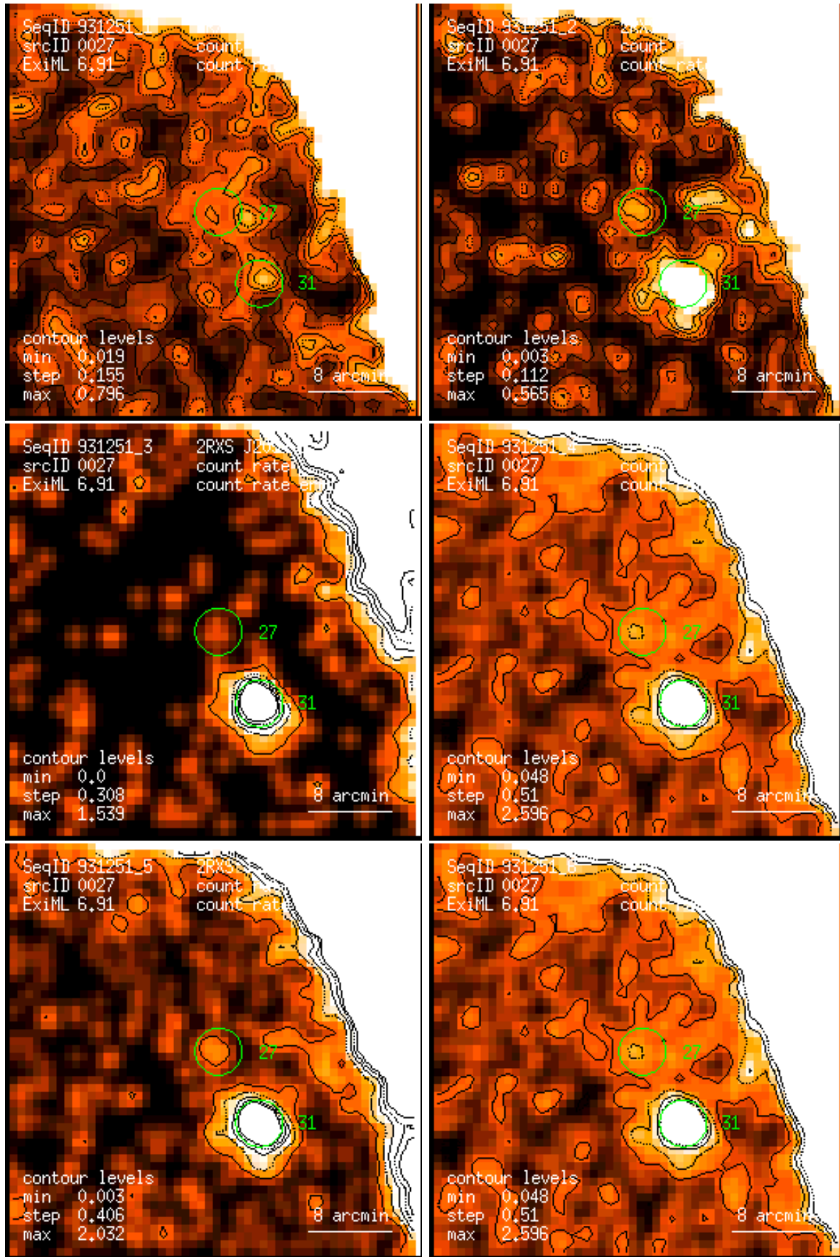
Figure 27: RASS 931251: detection 0027: band rate images, Gaussian filter: (1) PSPC channels 11 – 41, (2) 52 – 90, (3) 91 – 201, (4) 11 – 235, (5) 52 – 201, (6) 11 – 201. Broad band rates in counts/ks. Band rate contour levels in counts/ks/arcmin 2 .
