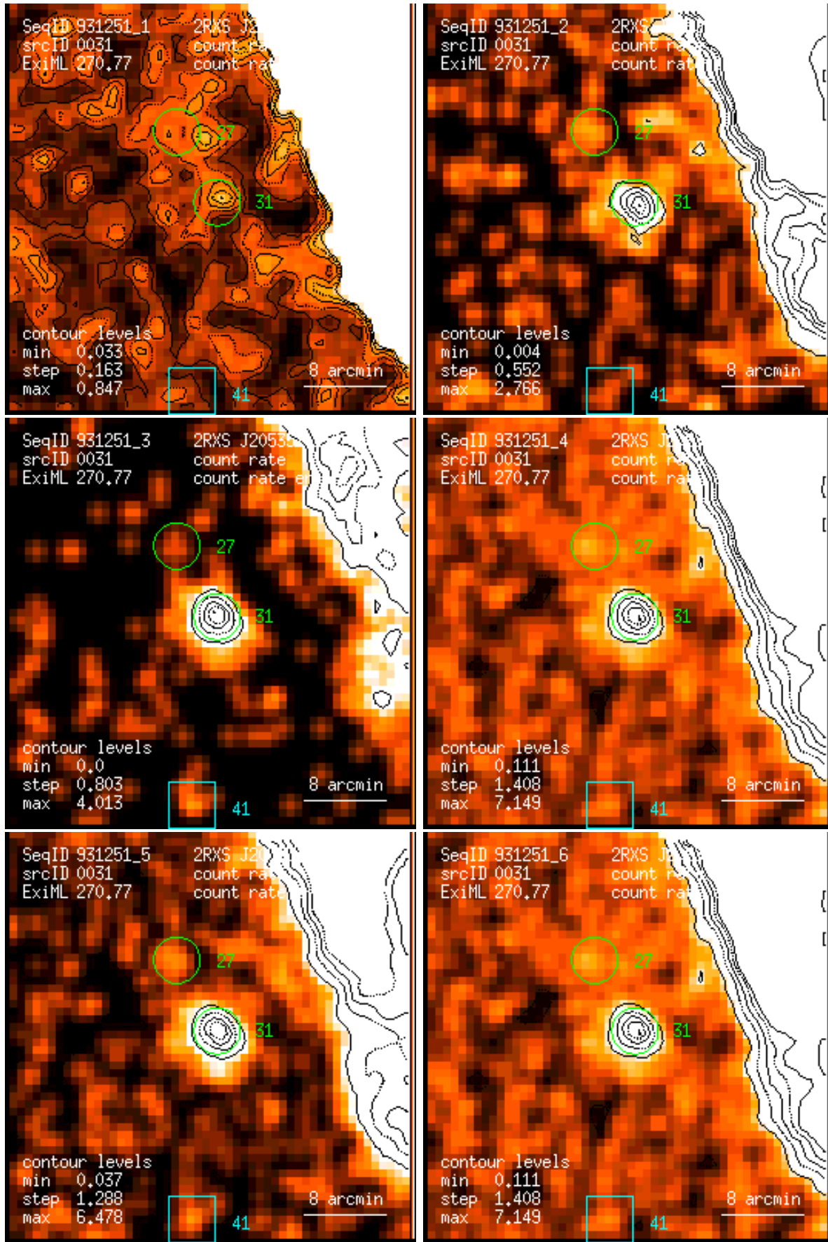
Figure 31: RASS 931251: detection 0031: band rate images, Gaussian filter: (1) PSPC channels 11 – 41, (2) 52 – 90, (3) 91 – 201, (4) 11 – 235, (5) 52 – 201, (6) 11 – 201. Broad band rates in counts/ks. Band rate contour levels in counts/ks/arcmin 2 .
