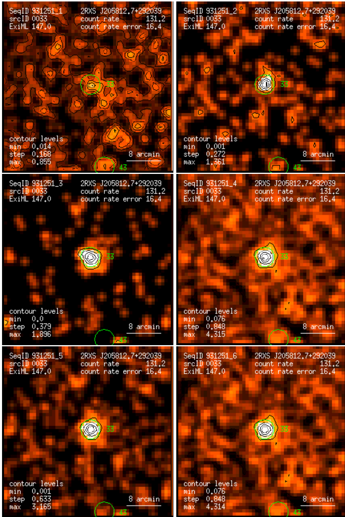
Figure 33: RASS 931251: detection 0033: band rate images, Gaussian filter: (1) PSPC channels 11 – 41, (2) 52 – 90, (3) 91 – 201, (4) 11 – 235, (5) 52 – 201, (6) 11 – 201. Broad band rates in counts/ks. Band rate contour levels in counts/ks/arcmin 2 .
