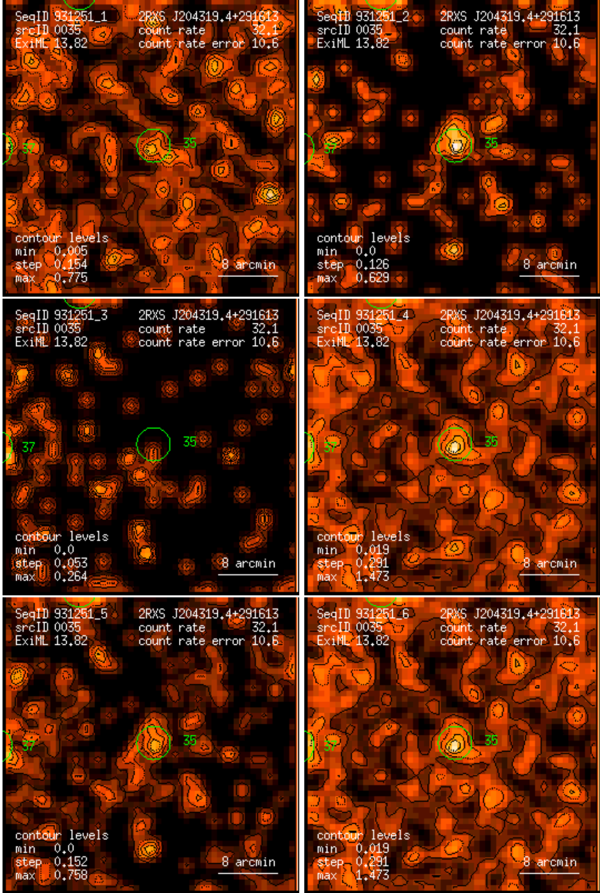
Figure 35: RASS 931251: detection 0035: band rate images, Gaussian filter: (1) PSPC channels 11 – 41, (2) 52 – 90, (3) 91 – 201, (4) 11 – 235, (5) 52 – 201, (6) 11 – 201. Broad band rates in counts/ks. Band rate contour levels in counts/ks/arcmin 2 .
