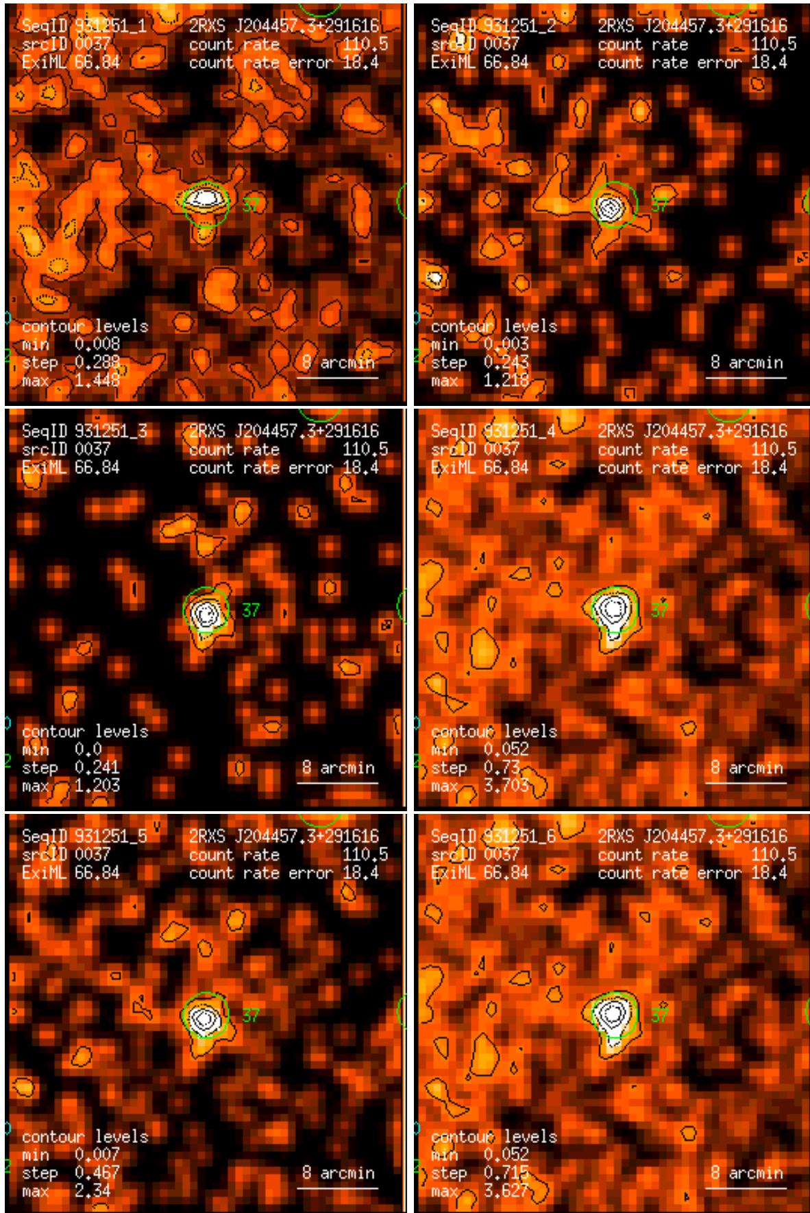
Figure 37: RASS 931251: detection 0037: band rate images, Gaussian filter: (1) PSPC channels 11 – 41, (2) 52 – 90, (3) 91 – 201, (4) 11 – 235, (5) 52 – 201, (6) 11 – 201. Broad band rates in counts/ks. Band rate contour levels in counts/ks/arcmin 2 .
