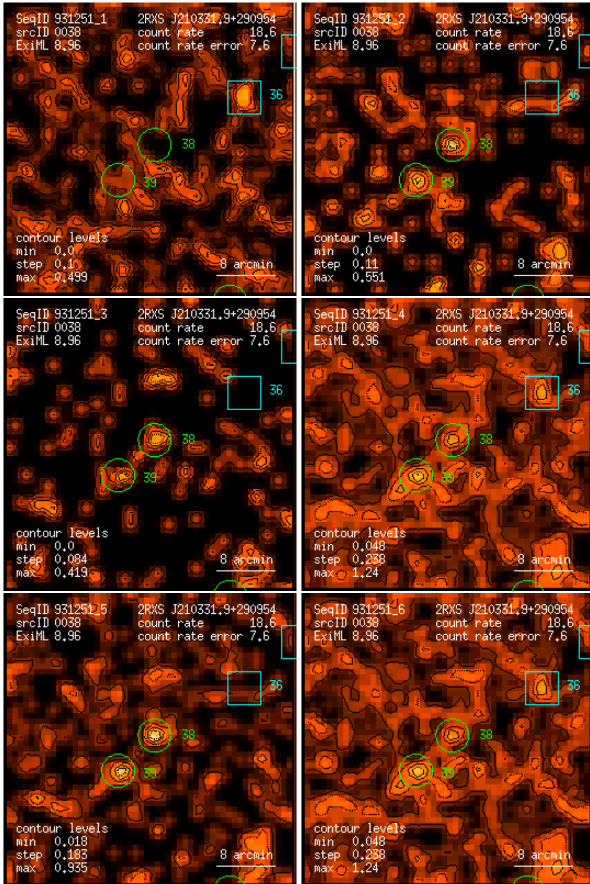
Figure 38: RASS 931251: detection 0038: band rate images, Gaussian filter: (1) PSPC channels 11 – 41, (2) 52 – 90, (3) 91 – 201, (4) 11 – 235, (5) 52 – 201, (6) 11 – 201. Broad band rates in counts/ks. Band rate contour levels in counts/ks/arcmin 2 .
