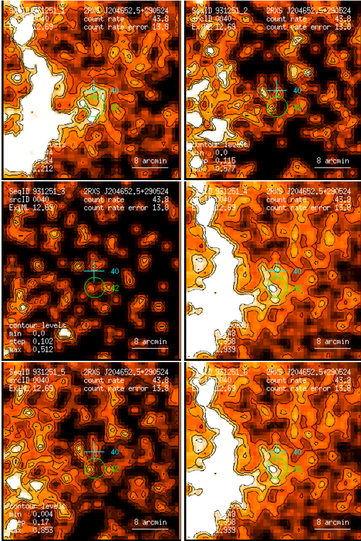
Figure 40: RASS 931251: detection 0040: band rate images, Gaussian filter: (1) PSPC channels 11 – 41, (2) 52 – 90, (3) 91 – 201, (4) 11 – 235, (5) 52 – 201, (6) 11 – 201. Broad band rates in counts/ks. Band rate contour levels in counts/ks/arcmin 2 .
