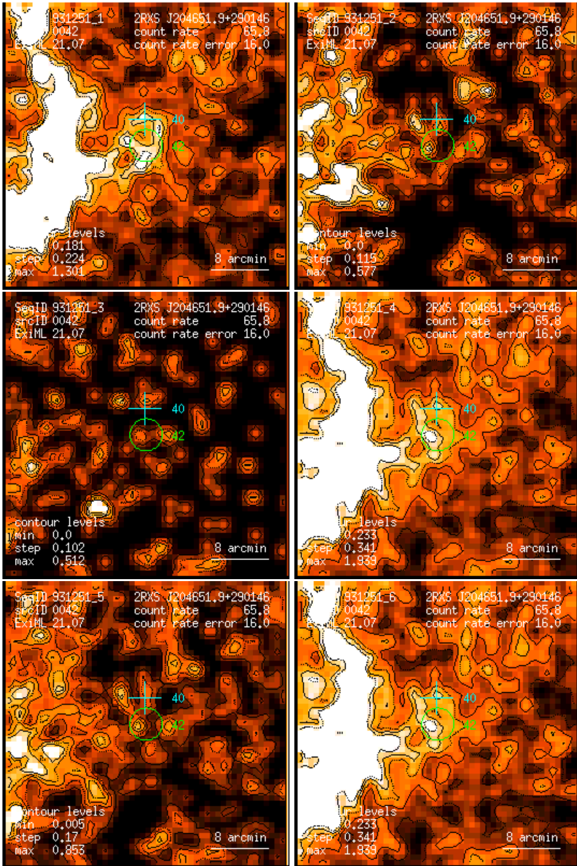
Figure 42: RASS 931251: detection 0042: band rate images, Gaussian filter: (1) PSPC channels 11 – 41, (2) 52 – 90, (3) 91 – 201, (4) 11 – 235, (5) 52 – 201, (6) 11 – 201. Broad band rates in counts/ks. Band rate contour levels in counts/ks/arcmin 2 .
