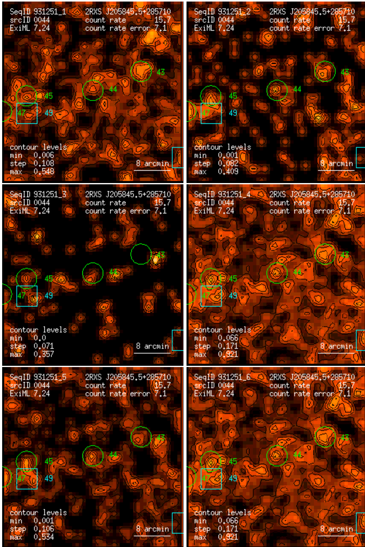
Figure 44: RASS 931251: detection 0044: band rate images, Gaussian filter: (1) PSPC channels 11 – 41, (2) 52 – 90, (3) 91 – 201, (4) 11 – 235, (5) 52 – 201, (6) 11 – 201. Broad band rates in counts/ks. Band rate contour levels in counts/ks/arcmin 2 .
