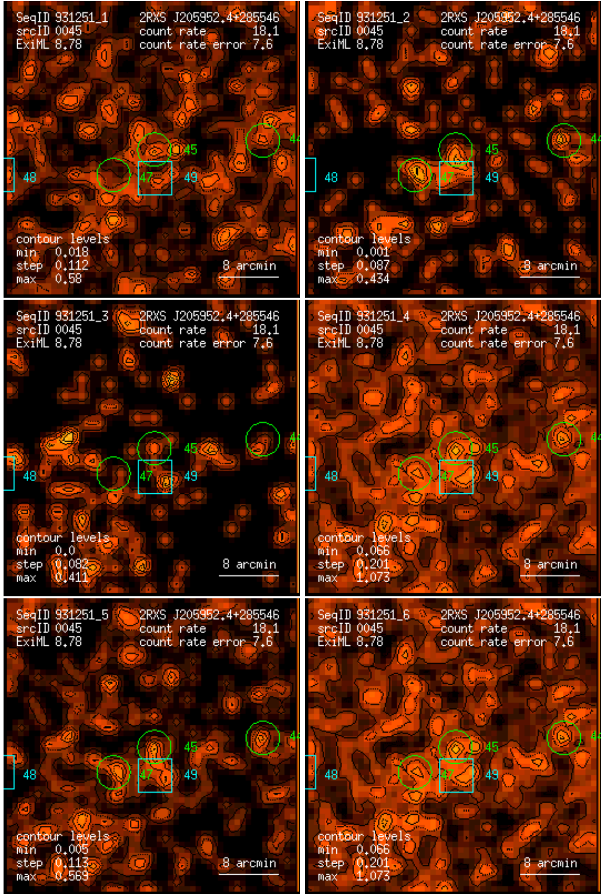
Figure 45: RASS 931251: detection 0045: band rate images, Gaussian filter: (1) PSPC channels 11 – 41, (2) 52 – 90, (3) 91 – 201, (4) 11 – 235, (5) 52 – 201, (6) 11 – 201. Broad band rates in counts/ks. Band rate contour levels in counts/ks/arcmin 2 .
