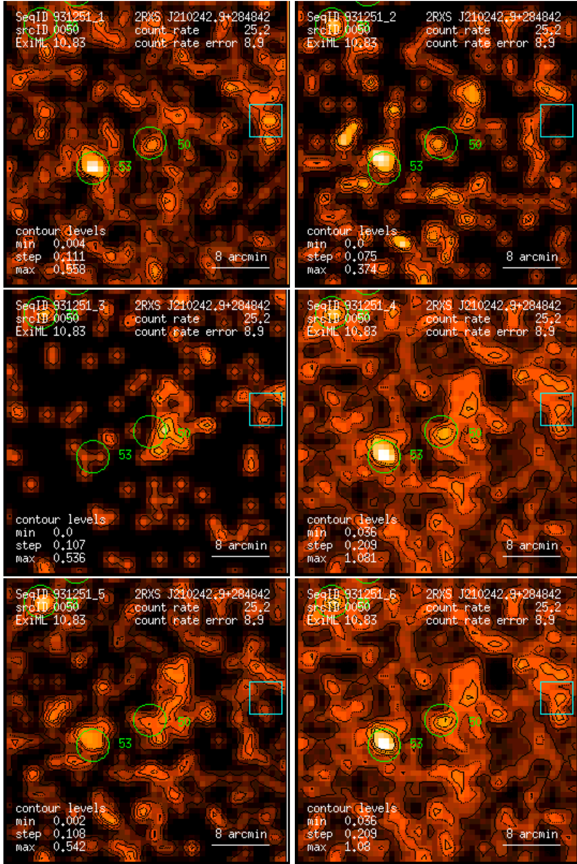
Figure 50: RASS 931251: detection 0050: band rate images, Gaussian filter: (1) PSPC channels 11 – 41, (2) 52 – 90, (3) 91 – 201, (4) 11 – 235, (5) 52 – 201, (6) 11 – 201. Broad band rates in counts/ks. Band rate contour levels in counts/ks/arcmin 2 .
