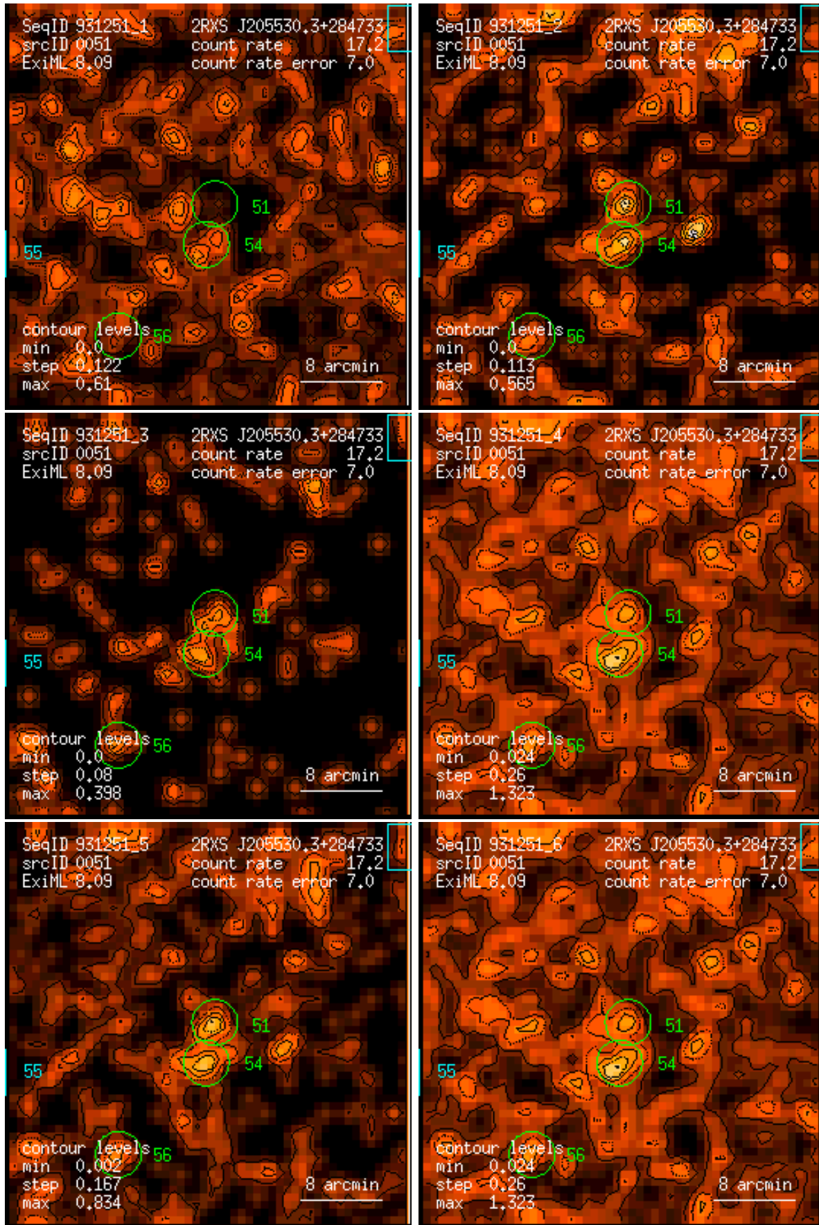
Figure 51: RASS 931251: detection 0051: band rate images, Gaussian filter: (1) PSPC channels 11 – 41, (2) 52 – 90, (3) 91 – 201, (4) 11 – 235, (5) 52 – 201, (6) 11 – 201. Broad band rates in counts/ks. Band rate contour levels in counts/ks/arcmin 2 .
