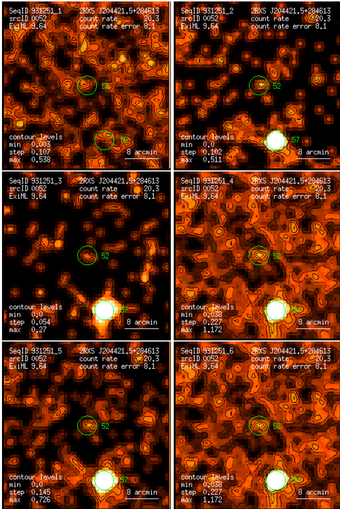
Figure 52: RASS 931251: detection 0052: band rate images, Gaussian filter: (1) PSPC channels 11 – 41, (2) 52 – 90, (3) 91 – 201, (4) 11 – 235, (5) 52 – 201, (6) 11 – 201. Broad band rates in counts/ks. Band rate contour levels in counts/ks/arcmin 2 .
