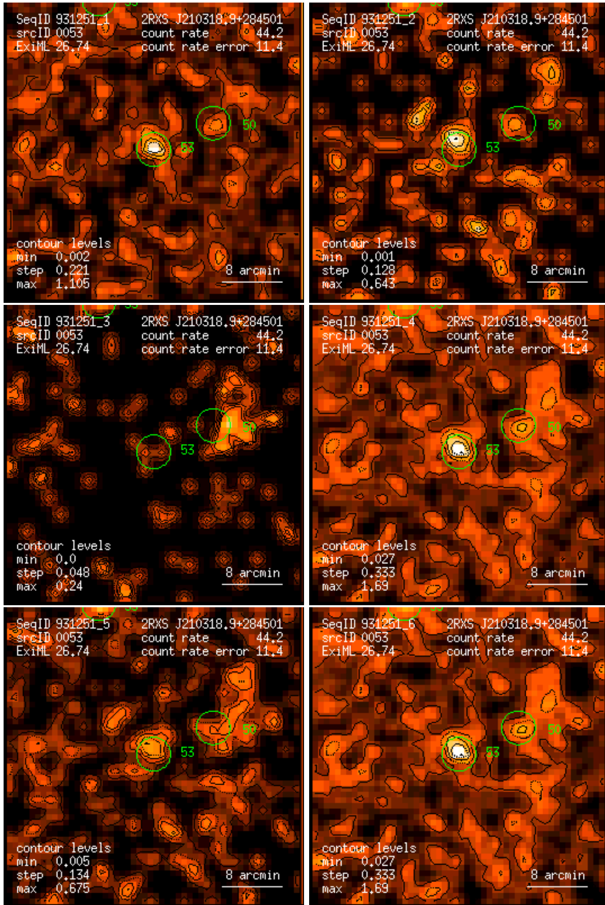
Figure 53: RASS 931251: detection 0053: band rate images, Gaussian filter: (1) PSPC channels 11 – 41, (2) 52 – 90, (3) 91 – 201, (4) 11 – 235, (5) 52 – 201, (6) 11 – 201. Broad band rates in counts/ks. Band rate contour levels in counts/ks/arcmin 2 .
