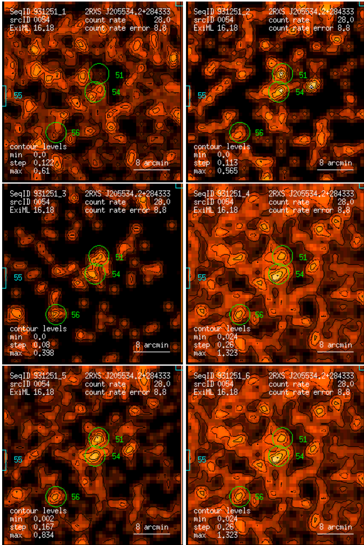
Figure 54: RASS 931251: detection 0054: band rate images, Gaussian filter: (1) PSPC channels 11 – 41, (2) 52 – 90, (3) 91 – 201, (4) 11 – 235, (5) 52 – 201, (6) 11 – 201. Broad band rates in counts/ks. Band rate contour levels in counts/ks/arcmin 2 .
