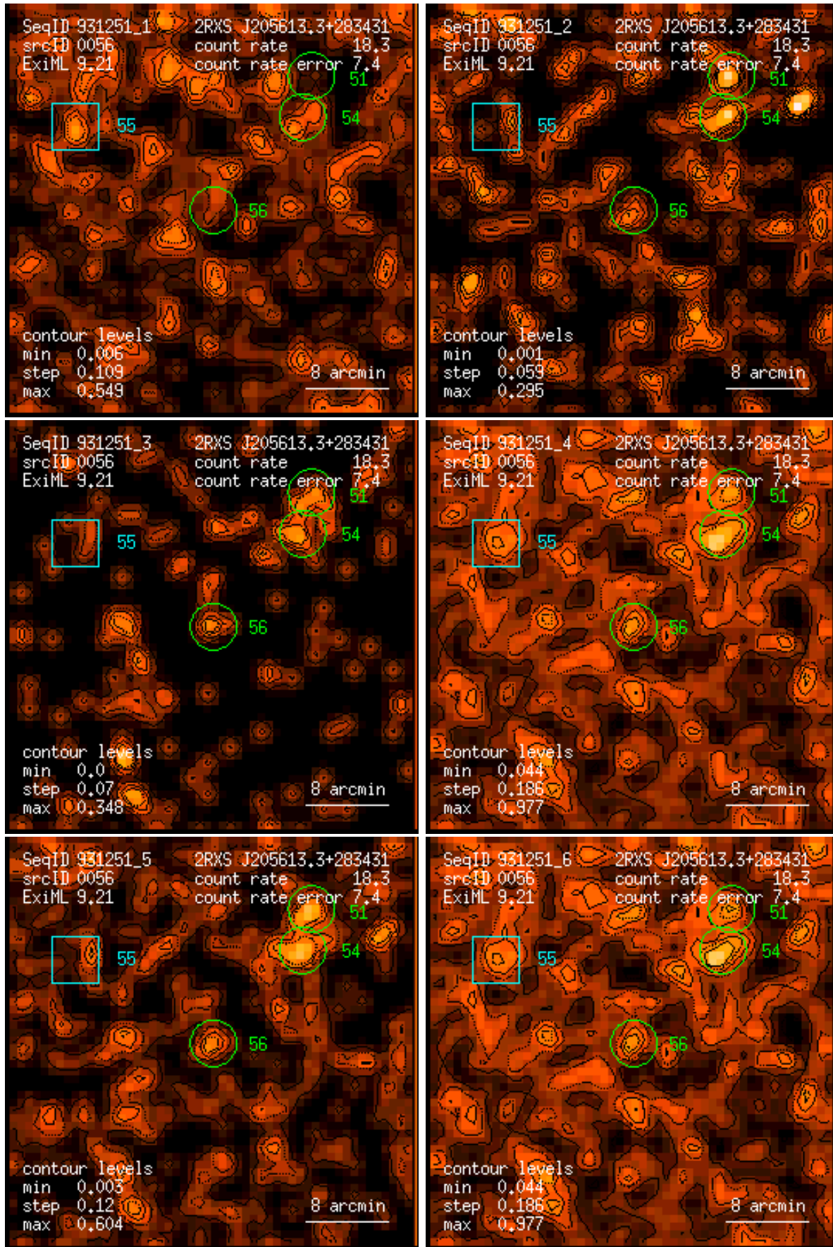
Figure 56: RASS 931251: detection 0056: band rate images, Gaussian filter: (1) PSPC channels 11 – 41, (2) 52 – 90, (3) 91 – 201, (4) 11 – 235, (5) 52 – 201, (6) 11 – 201. Broad band rates in counts/ks. Band rate contour levels in counts/ks/arcmin 2 .
