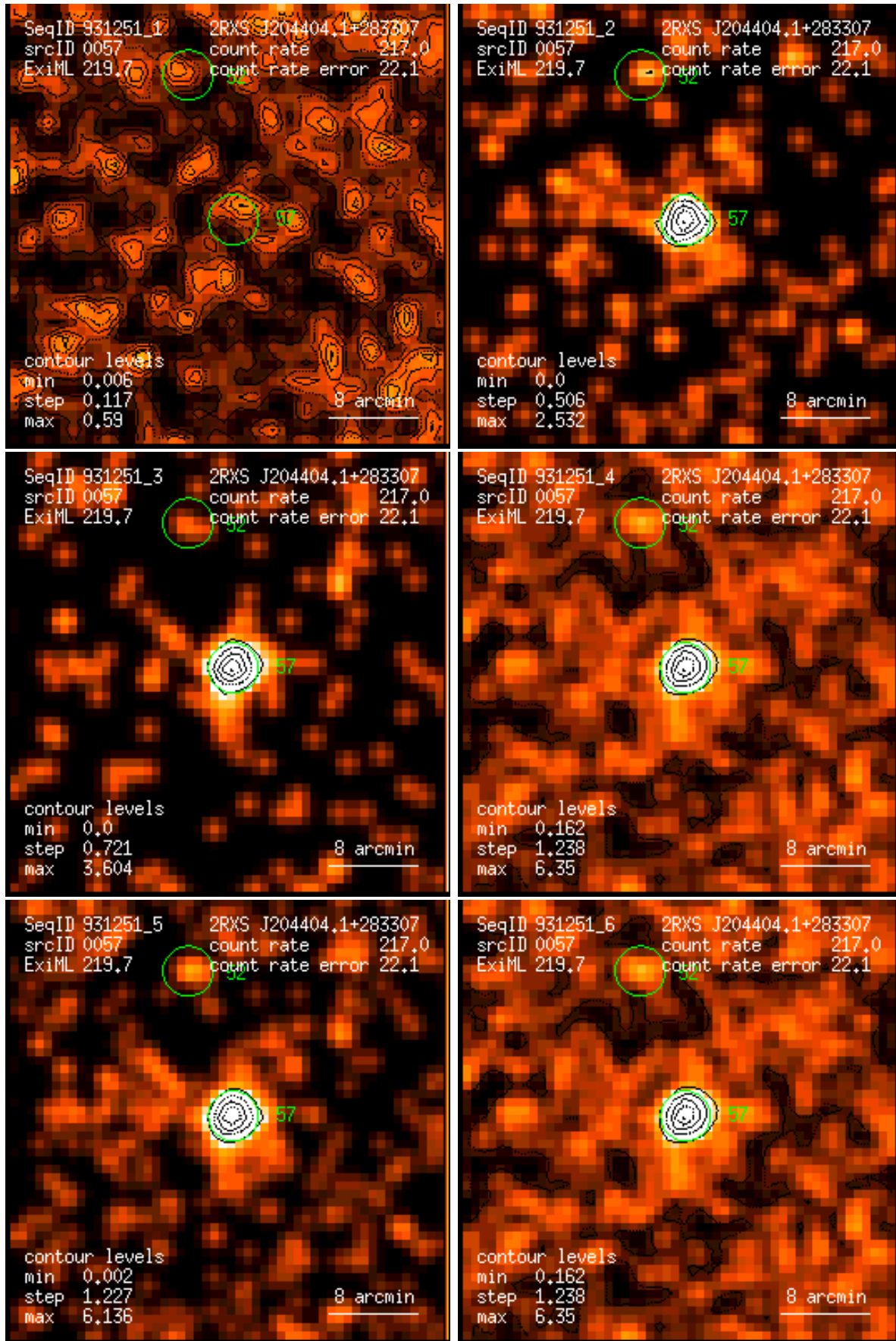
Figure 57: RASS 931251: detection 0057: band rate images, Gaussian filter: (1) PSPC channels 11 – 41, (2) 52 – 90, (3) 91 – 201, (4) 11 – 235, (5) 52 – 201, (6) 11 – 201. Broad band rates in counts/ks. Band rate contour levels in counts/ks/arcmin 2 .
