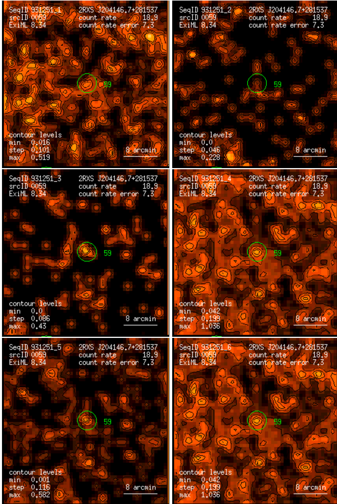
Figure 59: RASS 931251: detection 0059: band rate images, Gaussian filter: (1) PSPC channels 11 – 41, (2) 52 – 90, (3) 91 – 201, (4) 11 – 235, (5) 52 – 201, (6) 11 – 201. Broad band rates in counts/ks. Band rate contour levels in counts/ks/arcmin 2 .
