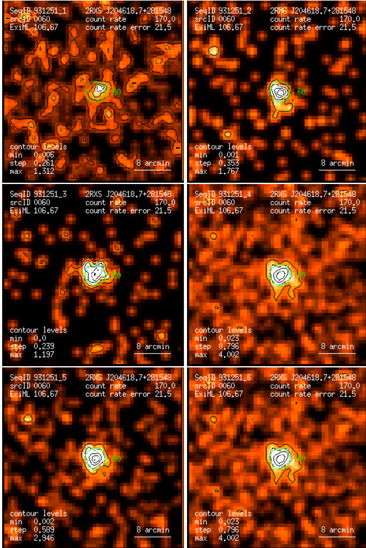
Figure 60: RASS 931251: detection 0060: band rate images, Gaussian filter: (1) PSPC channels 11 – 41, (2) 52 – 90, (3) 91 – 201, (4) 11 – 235, (5) 52 – 201, (6) 11 – 201. Broad band rates in counts/ks. Band rate contour levels in counts/ks/arcmin 2 .
