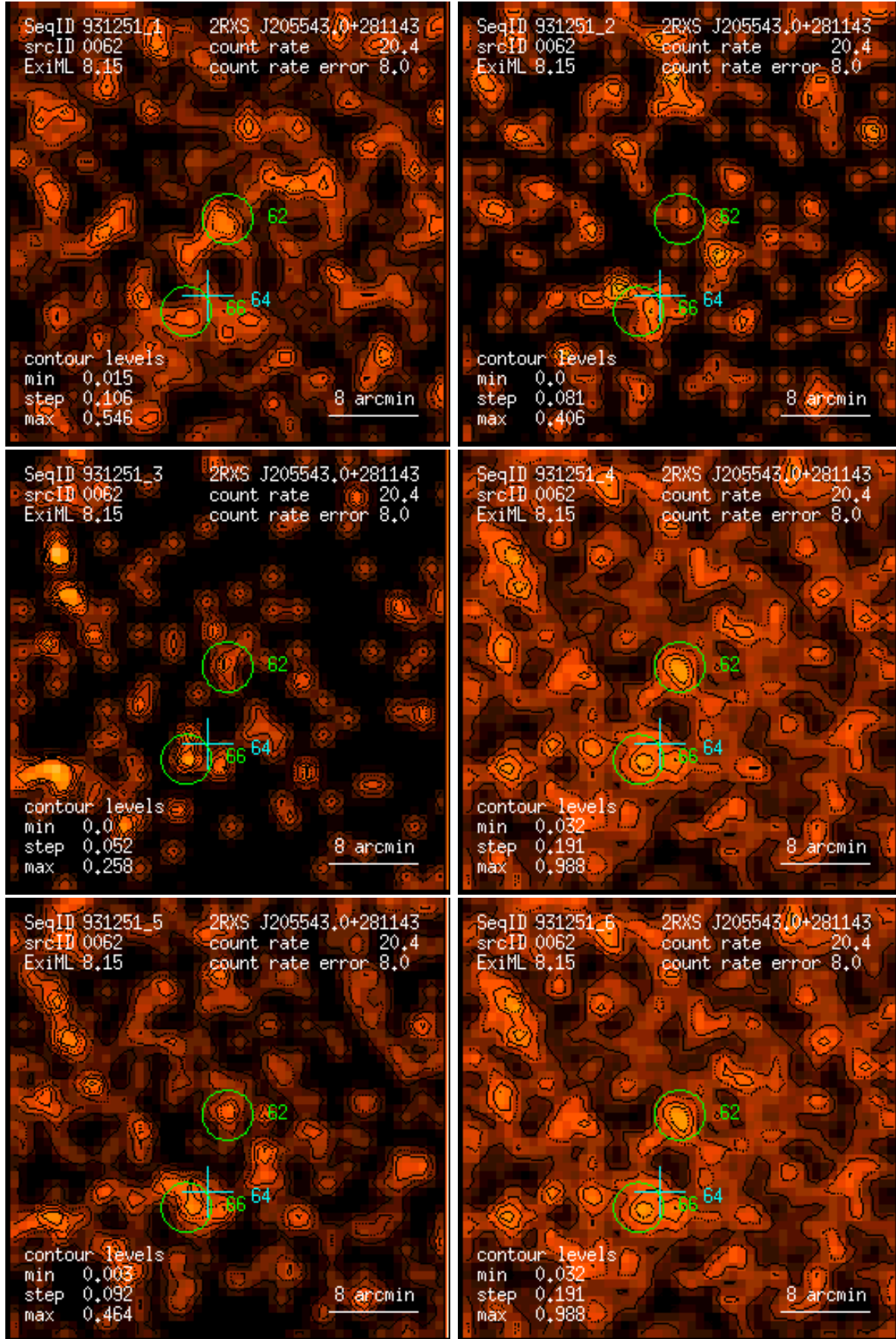
Figure 62: RASS 931251: detection 0062: band rate images, Gaussian filter: (1) PSPC channels 11 – 41, (2) 52 – 90, (3) 91 – 201, (4) 11 – 235, (5) 52 – 201, (6) 11 – 201. Broad band rates in counts/ks. Band rate contour levels in counts/ks/arcmin 2 .
