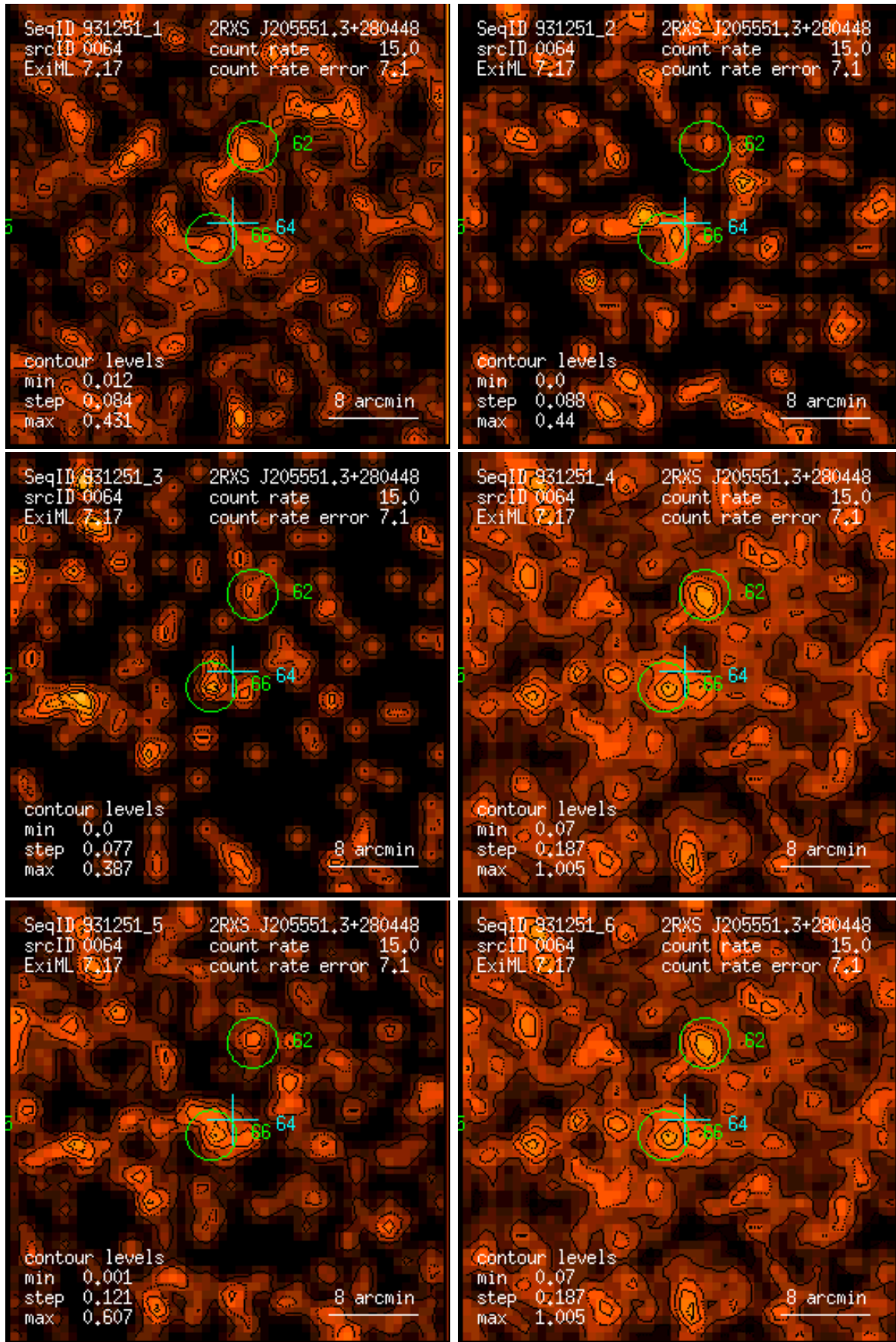
Figure 64: RASS 931251: detection 0064: band rate images, Gaussian filter: (1) PSPC channels 11 – 41, (2) 52 – 90, (3) 91 – 201, (4) 11 – 235, (5) 52 – 201, (6) 11 – 201. Broad band rates in counts/ks. Band rate contour levels in counts/ks/arcmin 2 .
