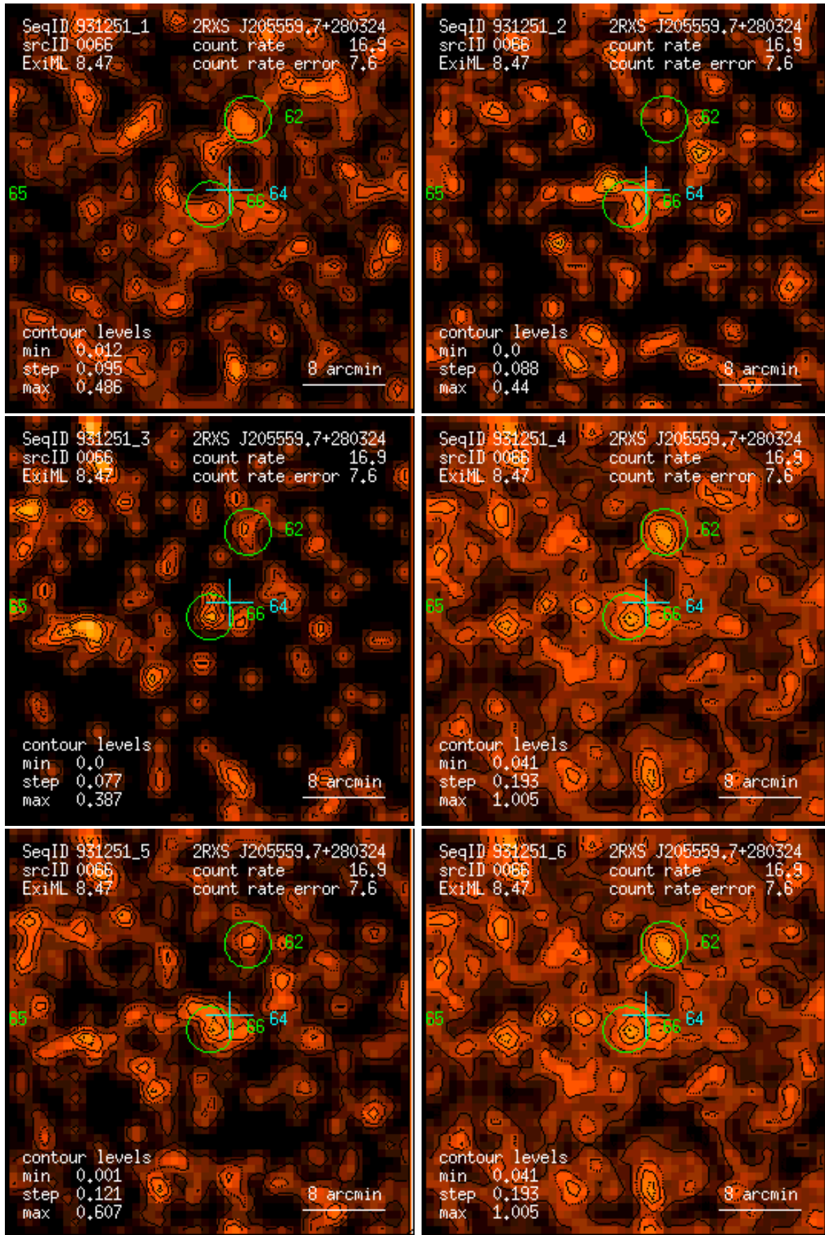
Figure 66: RASS 931251: detection 0066: band rate images, Gaussian filter: (1) PSPC channels 11 – 41, (2) 52 – 90, (3) 91 – 201, (4) 11 – 235, (5) 52 – 201, (6) 11 – 201. Broad band rates in counts/ks. Band rate contour levels in counts/ks/arcmin 2 .
