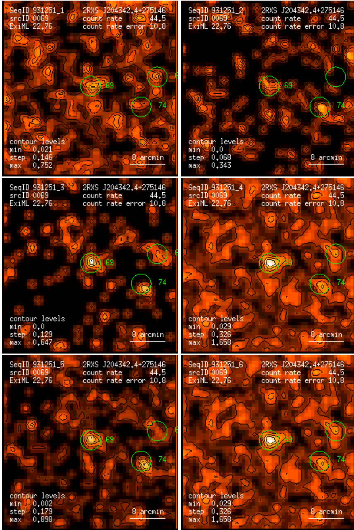
Figure 69: RASS 931251: detection 0069: band rate images, Gaussian filter: (1) PSPC channels 11 – 41, (2) 52 – 90, (3) 91 – 201, (4) 11 – 235, (5) 52 – 201, (6) 11 – 201. Broad band rates in counts/ks. Band rate contour levels in counts/ks/arcmin 2 .
