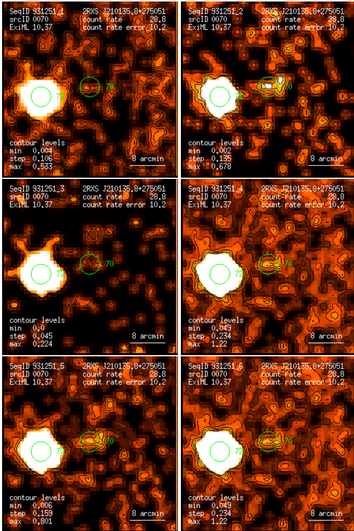
Figure 70: RASS 931251: detection 0070: band rate images, Gaussian filter: (1) PSPC channels 11 – 41, (2) 52 – 90, (3) 91 – 201, (4) 11 – 235, (5) 52 – 201, (6) 11 – 201. Broad band rates in counts/ks. Band rate contour levels in counts/ks/arcmin 2 .
