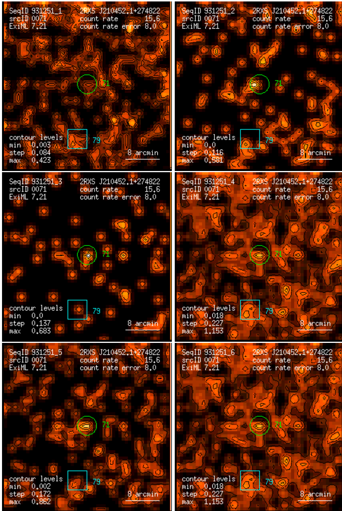
Figure 71: RASS 931251: detection 0071: band rate images, Gaussian filter: (1) PSPC channels 11 – 41, (2) 52 – 90, (3) 91 – 201, (4) 11 – 235, (5) 52 – 201, (6) 11 – 201. Broad band rates in counts/ks. Band rate contour levels in counts/ks/arcmin 2 .
