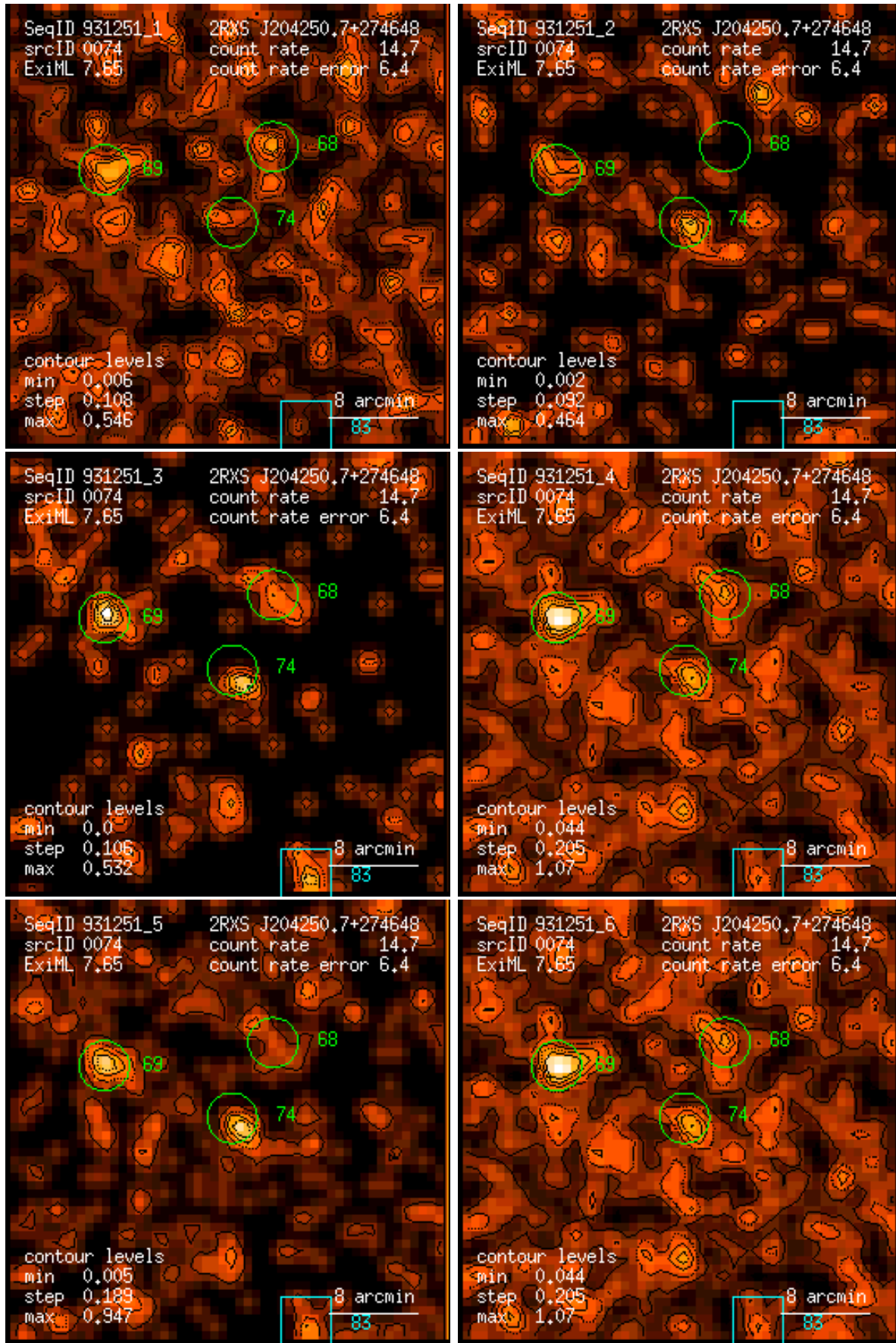
Figure 74: RASS 931251: detection 0074: band rate images, Gaussian filter: (1) PSPC channels 11 – 41, (2) 52 – 90, (3) 91 – 201, (4) 11 – 235, (5) 52 – 201, (6) 11 – 201. Broad band rates in counts/ks. Band rate contour levels in counts/ks/arcmin 2 .
