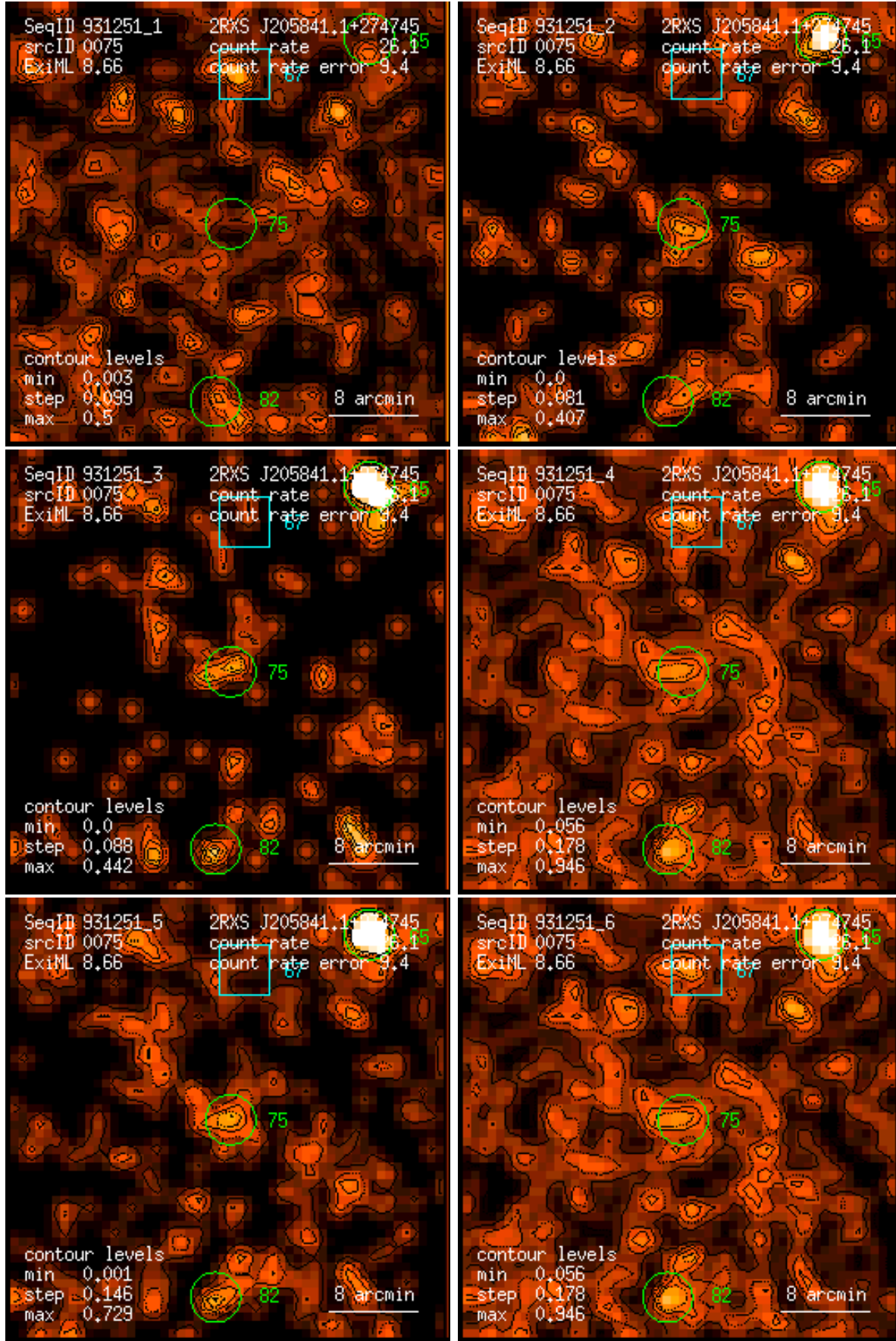
Figure 75: RASS 931251: detection 0075: band rate images, Gaussian filter: (1) PSPC channels 11 – 41, (2) 52 – 90, (3) 91 – 201, (4) 11 – 235, (5) 52 – 201, (6) 11 – 201. Broad band rates in counts/ks. Band rate contour levels in counts/ks/arcmin 2 .
