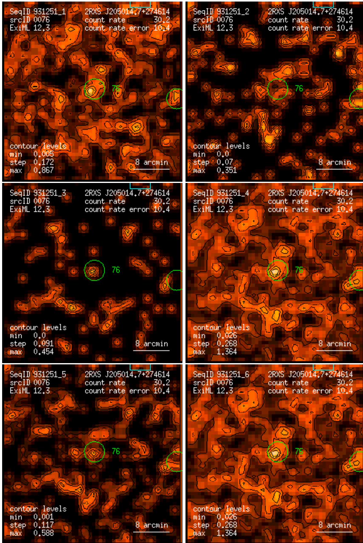
Figure 76: RASS 931251: detection 0076: band rate images, Gaussian filter: (1) PSPC channels 11 – 41, (2) 52 – 90, (3) 91 – 201, (4) 11 – 235, (5) 52 – 201, (6) 11 – 201. Broad band rates in counts/ks. Band rate contour levels in counts/ks/arcmin 2 .
