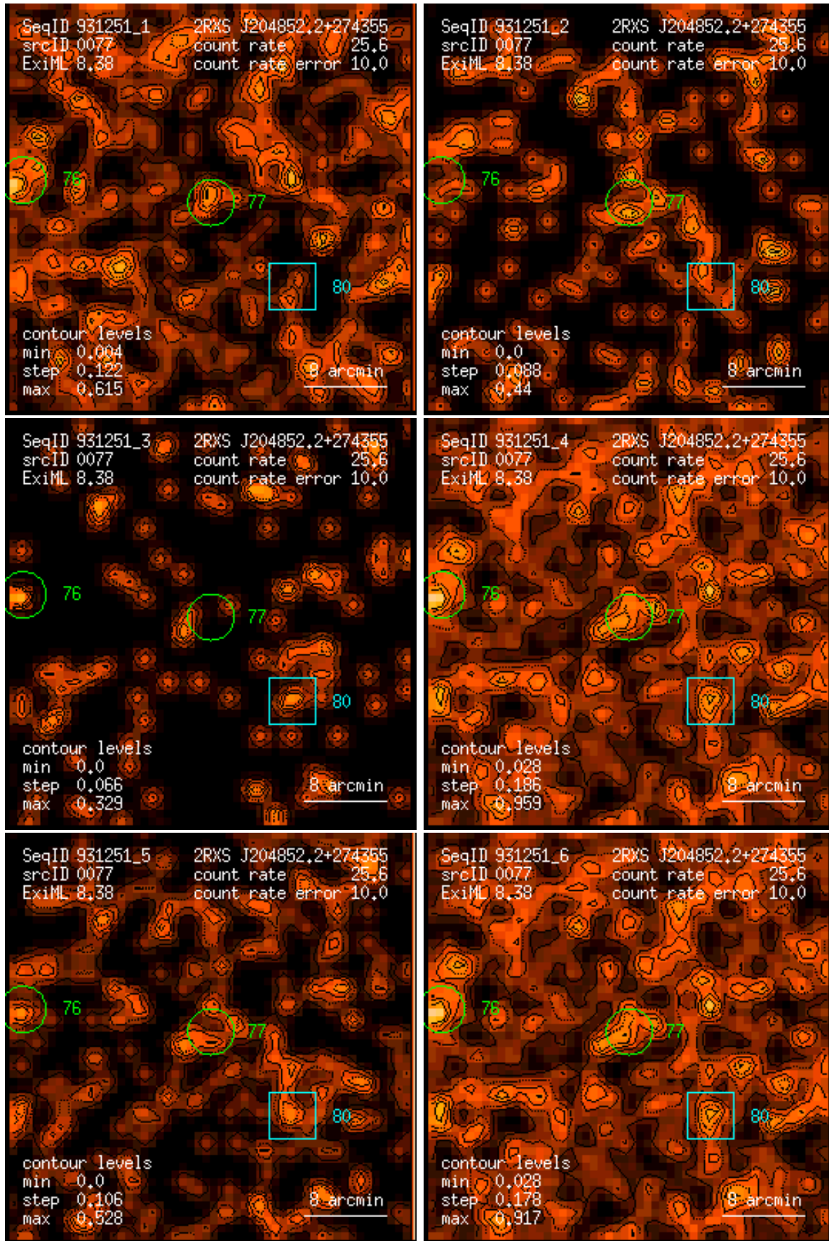
Figure 77: RASS 931251: detection 0077: band rate images, Gaussian filter: (1) PSPC channels 11 – 41, (2) 52 – 90, (3) 91 – 201, (4) 11 – 235, (5) 52 – 201, (6) 11 – 201. Broad band rates in counts/ks. Band rate contour levels in counts/ks/arcmin 2 .
