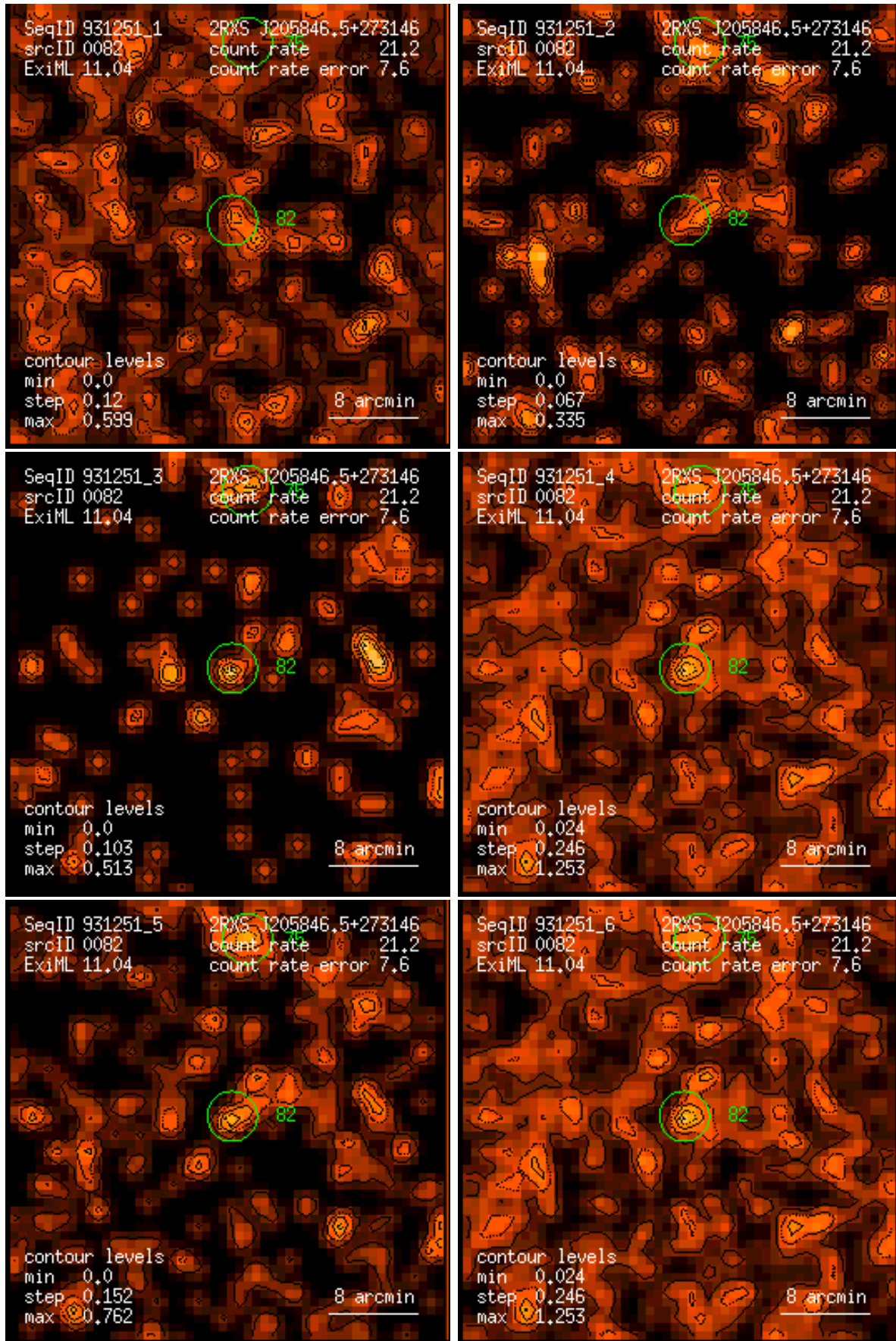
Figure 82: RASS 931251: detection 0082: band rate images, Gaussian filter: (1) PSPC channels 11 – 41, (2) 52 – 90, (3) 91 – 201, (4) 11 – 235, (5) 52 – 201, (6) 11 – 201. Broad band rates in counts/ks. Band rate contour levels in counts/ks/arcmin 2 .
