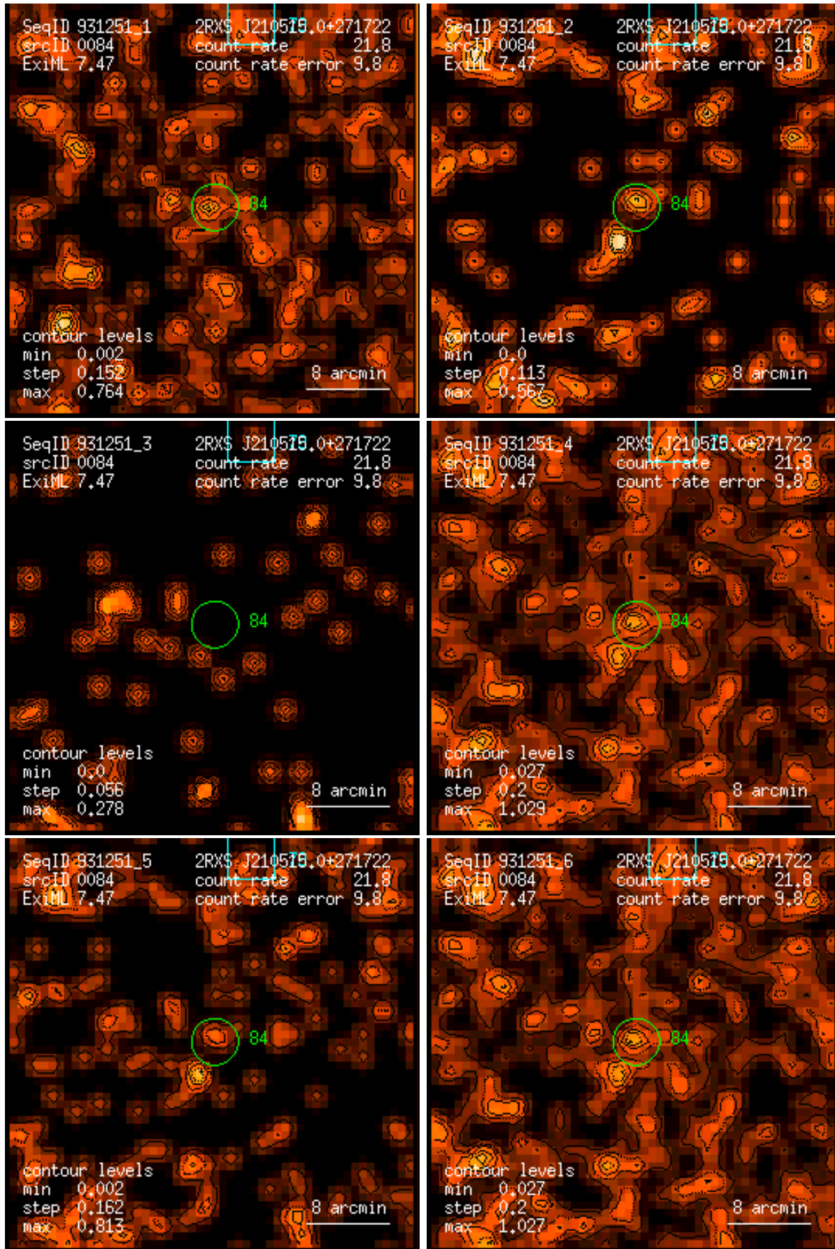
Figure 84: RASS 931251: detection 0084: band rate images, Gaussian filter: (1) PSPC channels 11 – 41, (2) 52 – 90, (3) 91 – 201, (4) 11 – 235, (5) 52 – 201, (6) 11 – 201. Broad band rates in counts/ks. Band rate contour levels in counts/ks/arcmin 2 .
